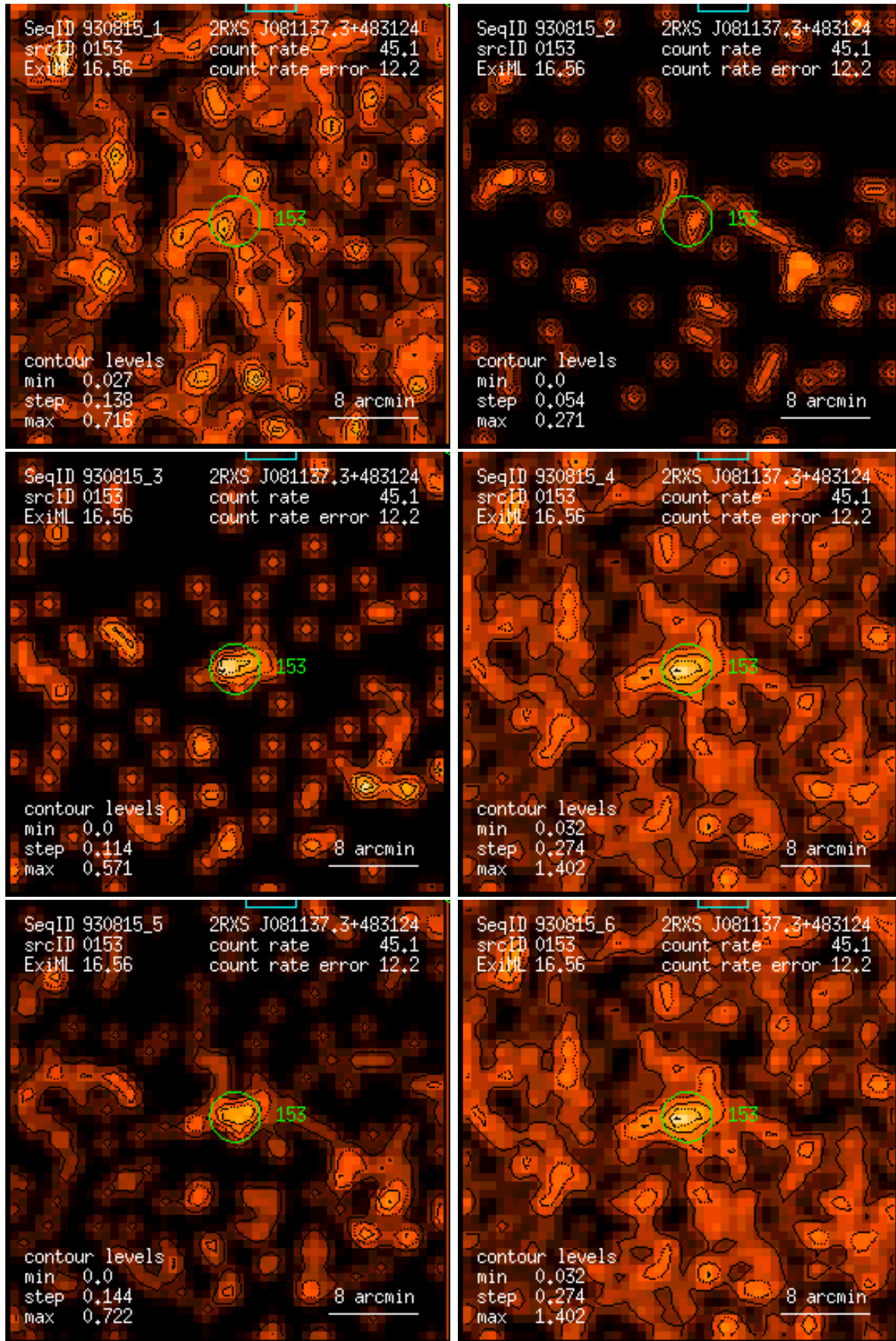
Figure 153: RASS 930815: detection 0153: band rate images, Gaussian filter: (1) PSPC channels 11 – 41, (2) 52 – 90, (3) 91 – 201, (4) 11 – 235, (5) 52 – 201, (6) 11 – 201. Broad band rates in counts/ks. Band rate contour levels in counts/ks/arcmin 2 .
