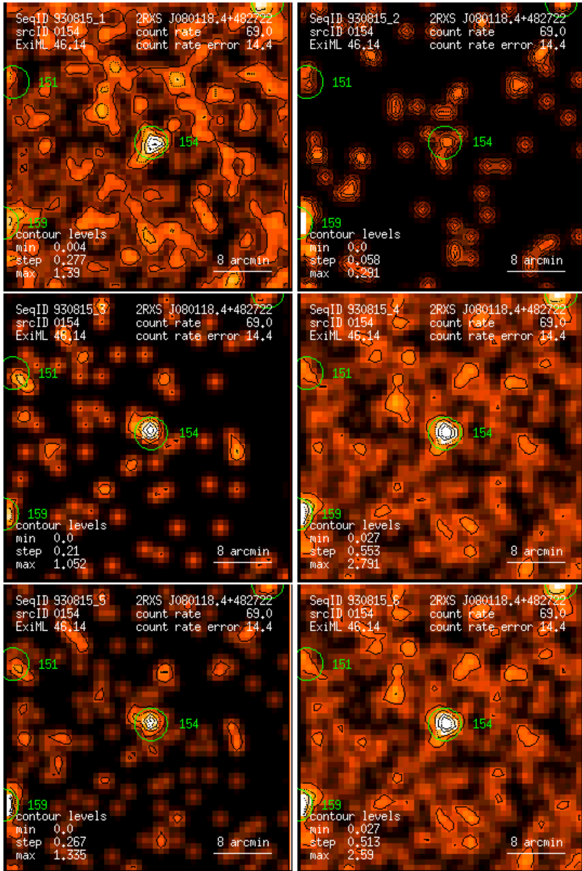
Figure 154: RASS 930815: detection 0154: band rate images, Gaussian filter: (1) PSPC channels 11 – 41, (2) 52 – 90, (3) 91 – 201, (4) 11 – 235, (5) 52 – 201, (6) 11 – 201. Broad band rates in counts/ks. Band rate contour levels in counts/ks/arcmin 2 .
