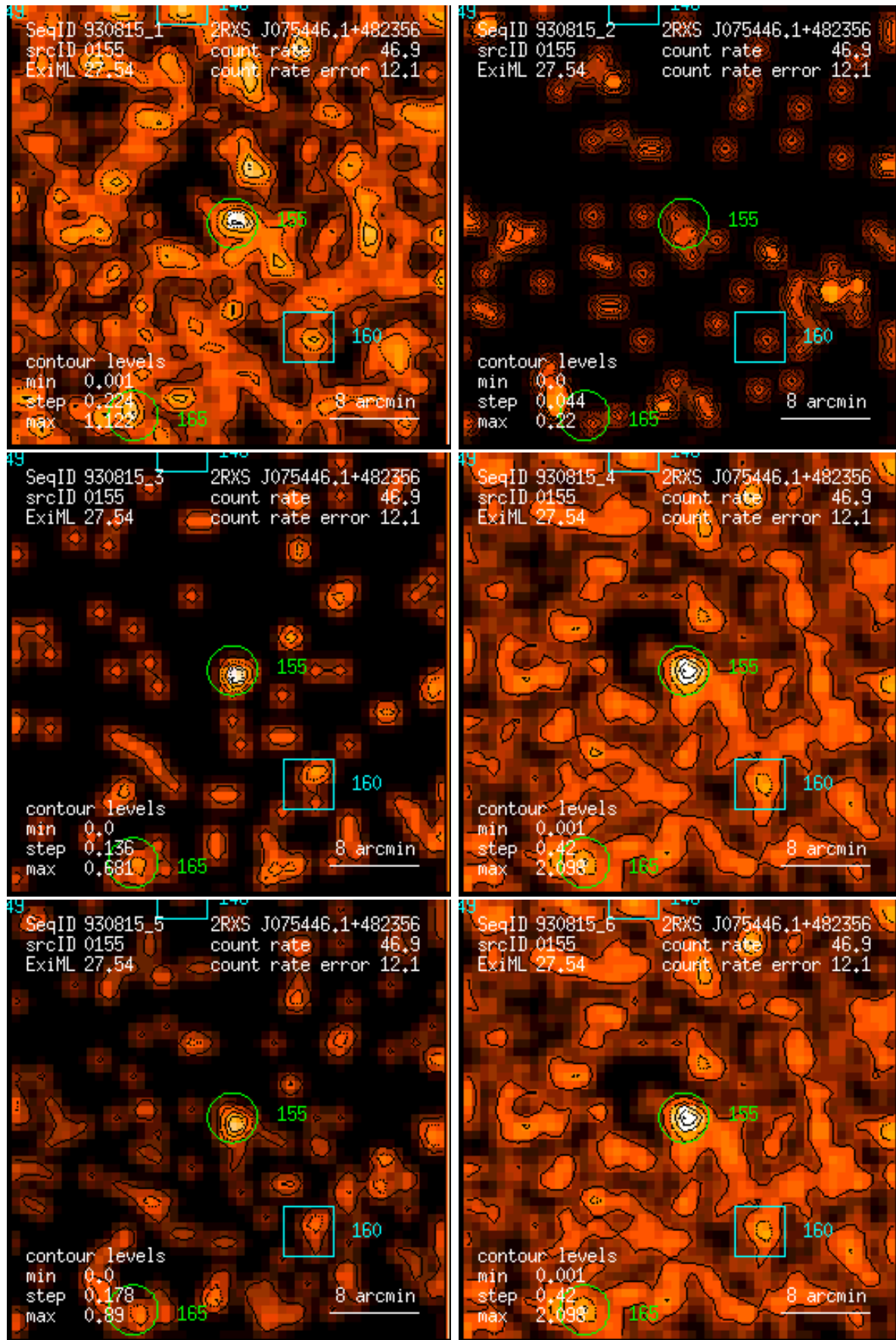
Figure 155: RASS 930815: detection 0155: band rate images, Gaussian filter: (1) PSPC channels 11 – 41, (2) 52 – 90, (3) 91 – 201, (4) 11 – 235, (5) 52 – 201, (6) 11 – 201. Broad band rates in counts/ks. Band rate contour levels in counts/ks/arcmin 2 .
