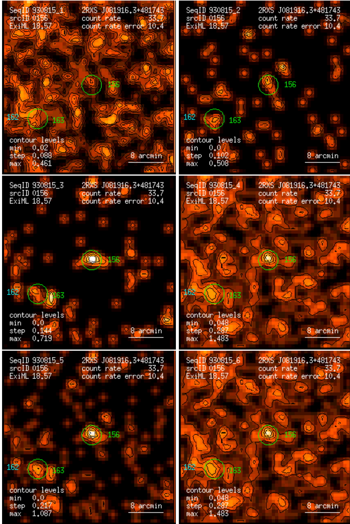
Figure 156: RASS 930815: detection 0156: band rate images, Gaussian filter: (1) PSPC channels 11 – 41, (2) 52 – 90, (3) 91 – 201, (4) 11 – 235, (5) 52 – 201, (6) 11 – 201. Broad band rates in counts/ks. Band rate contour levels in counts/ks/arcmin 2 .
