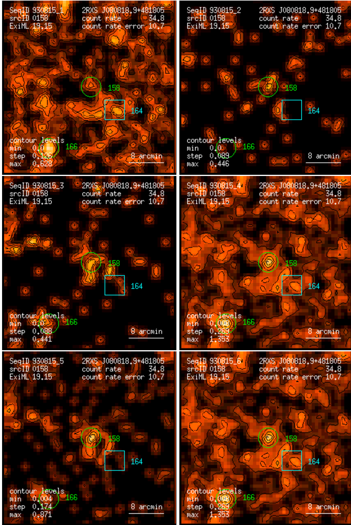
Figure 158: RASS 930815: detection 0158: band rate images, Gaussian filter: (1) PSPC channels 11 – 41, (2) 52 – 90, (3) 91 – 201, (4) 11 – 235, (5) 52 – 201, (6) 11 – 201. Broad band rates in counts/ks. Band rate contour levels in counts/ks/arcmin 2 .
