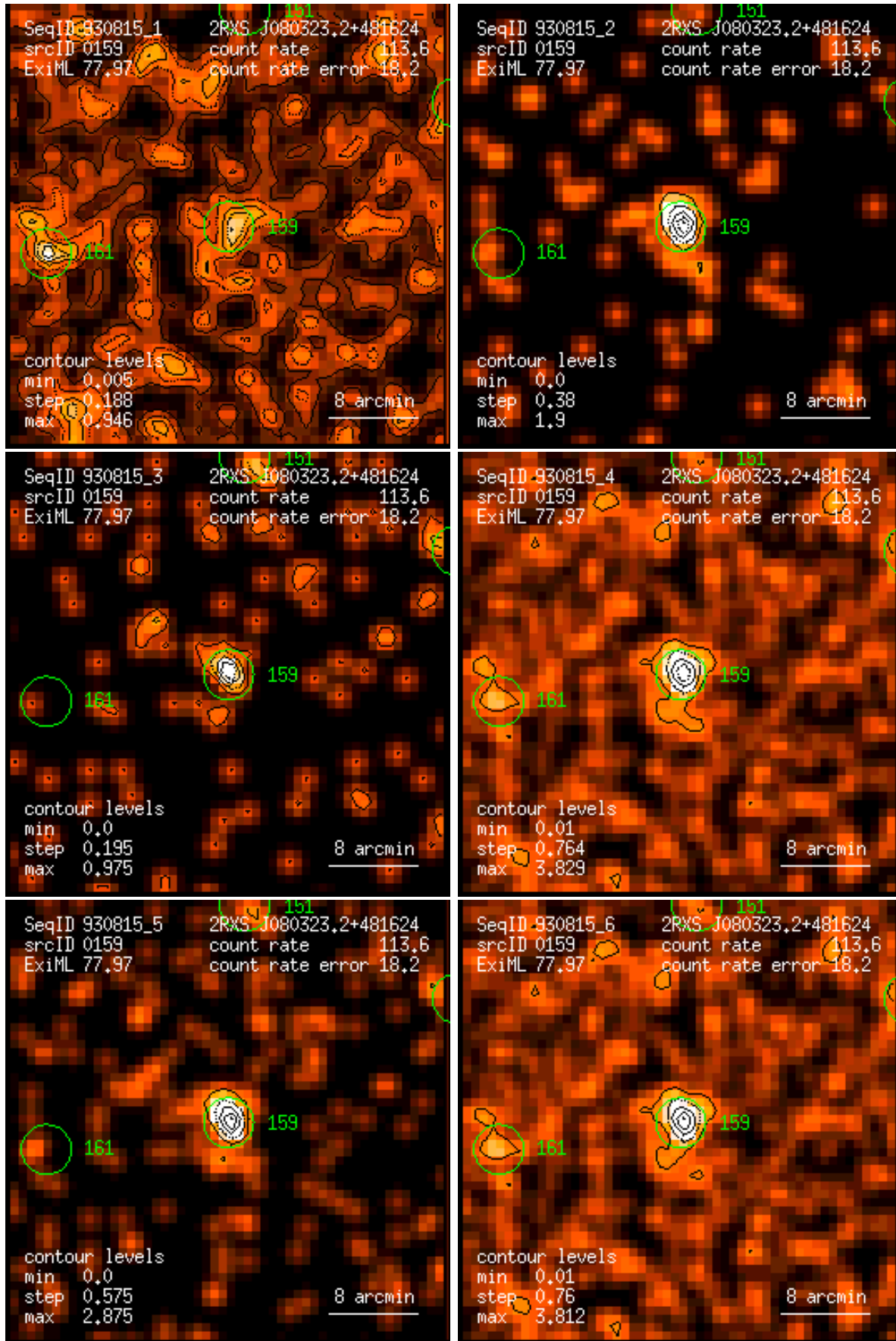
Figure 159: RASS 930815: detection 0159: band rate images, Gaussian filter: (1) PSPC channels 11 – 41, (2) 52 – 90, (3) 91 – 201, (4) 11 – 235, (5) 52 – 201, (6) 11 – 201. Broad band rates in counts/ks. Band rate contour levels in counts/ks/arcmin 2 .
