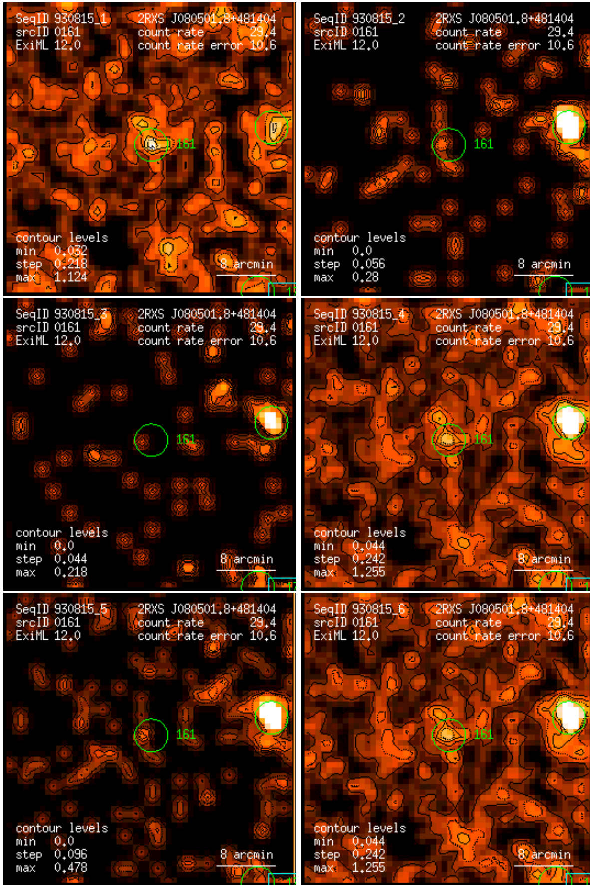
Figure 161: RASS 930815: detection 0161: band rate images, Gaussian filter: (1) PSPC channels 11 – 41, (2) 52 – 90, (3) 91 – 201, (4) 11 – 235, (5) 52 – 201, (6) 11 – 201. Broad band rates in counts/ks. Band rate contour levels in counts/ks/arcmin 2 .
