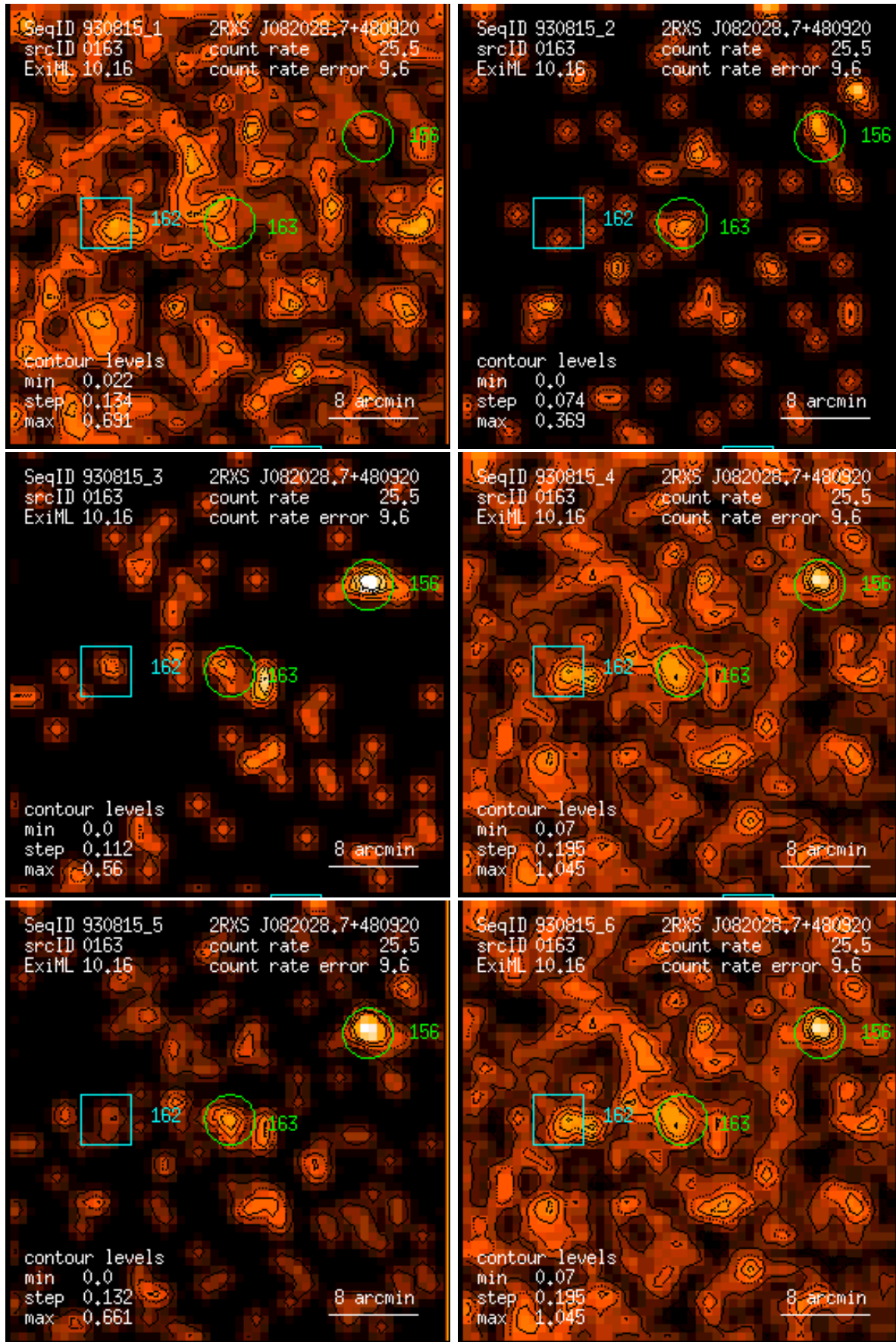
Figure 163: RASS 930815: detection 0163: band rate images, Gaussian filter: (1) PSPC channels 11 – 41, (2) 52 – 90, (3) 91 – 201, (4) 11 – 235, (5) 52 – 201, (6) 11 – 201. Broad band rates in counts/ks. Band rate contour levels in counts/ks/arcmin 2 .
