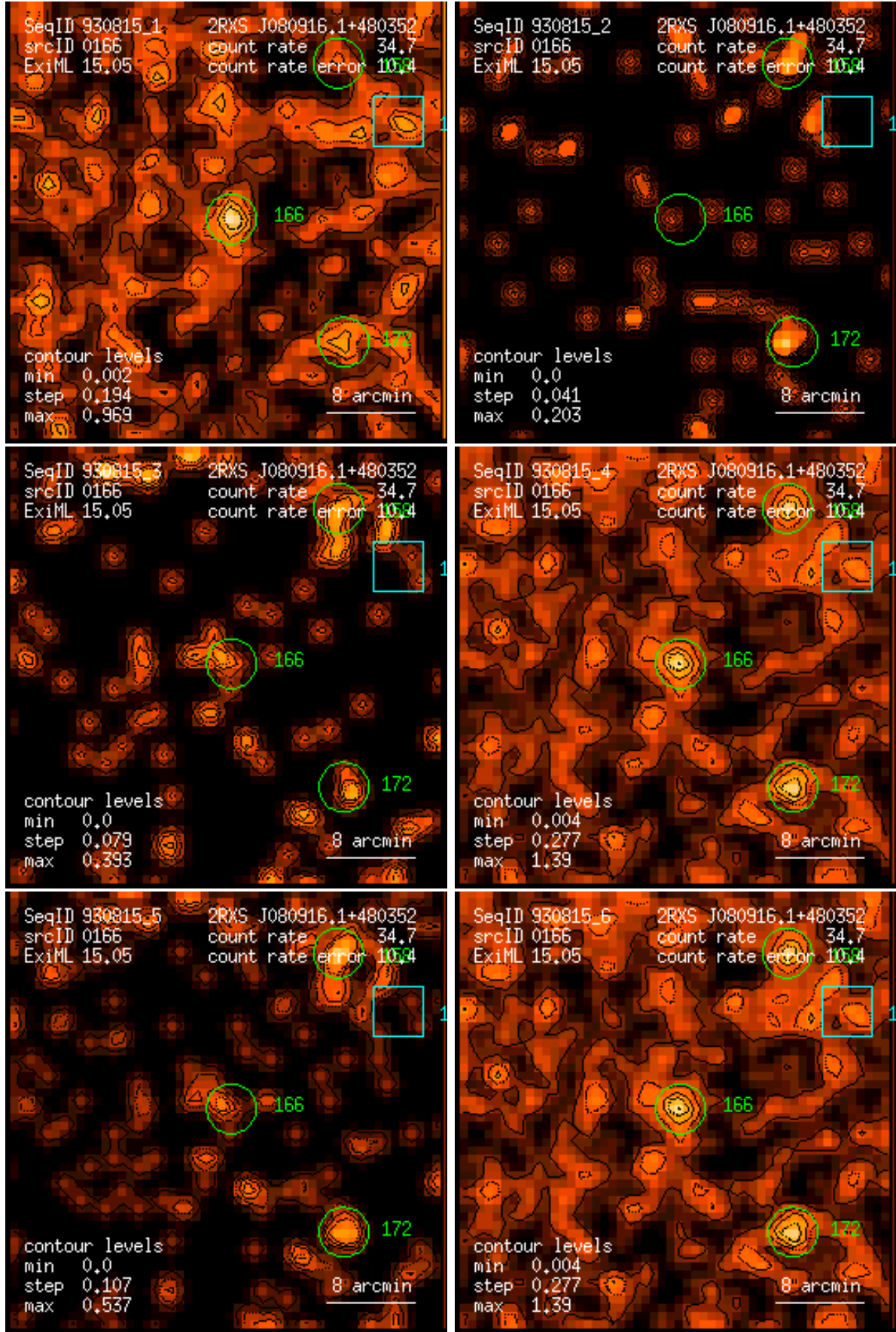
Figure 166: RASS 930815: detection 0166: band rate images, Gaussian filter: (1) PSPC channels 11 – 41, (2) 52 – 90, (3) 91 – 201, (4) 11 – 235, (5) 52 – 201, (6) 11 – 201. Broad band rates in counts/ks. Band rate contour levels in counts/ks/arcmin 2 .
