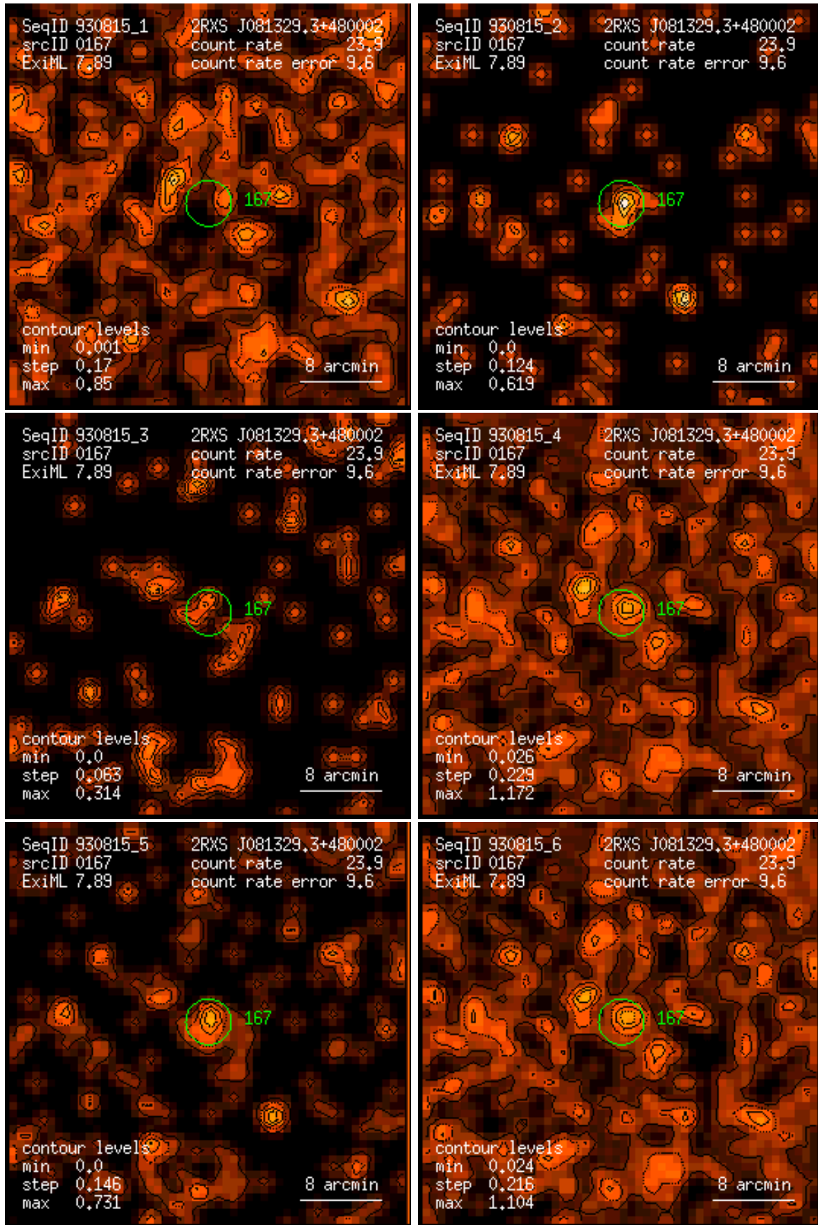
Figure 167: RASS 930815: detection 0167: band rate images, Gaussian filter: (1) PSPC channels 11 – 41, (2) 52 – 90, (3) 91 – 201, (4) 11 – 235, (5) 52 – 201, (6) 11 – 201. Broad band rates in counts/ks. Band rate contour levels in counts/ks/arcmin 2 .
