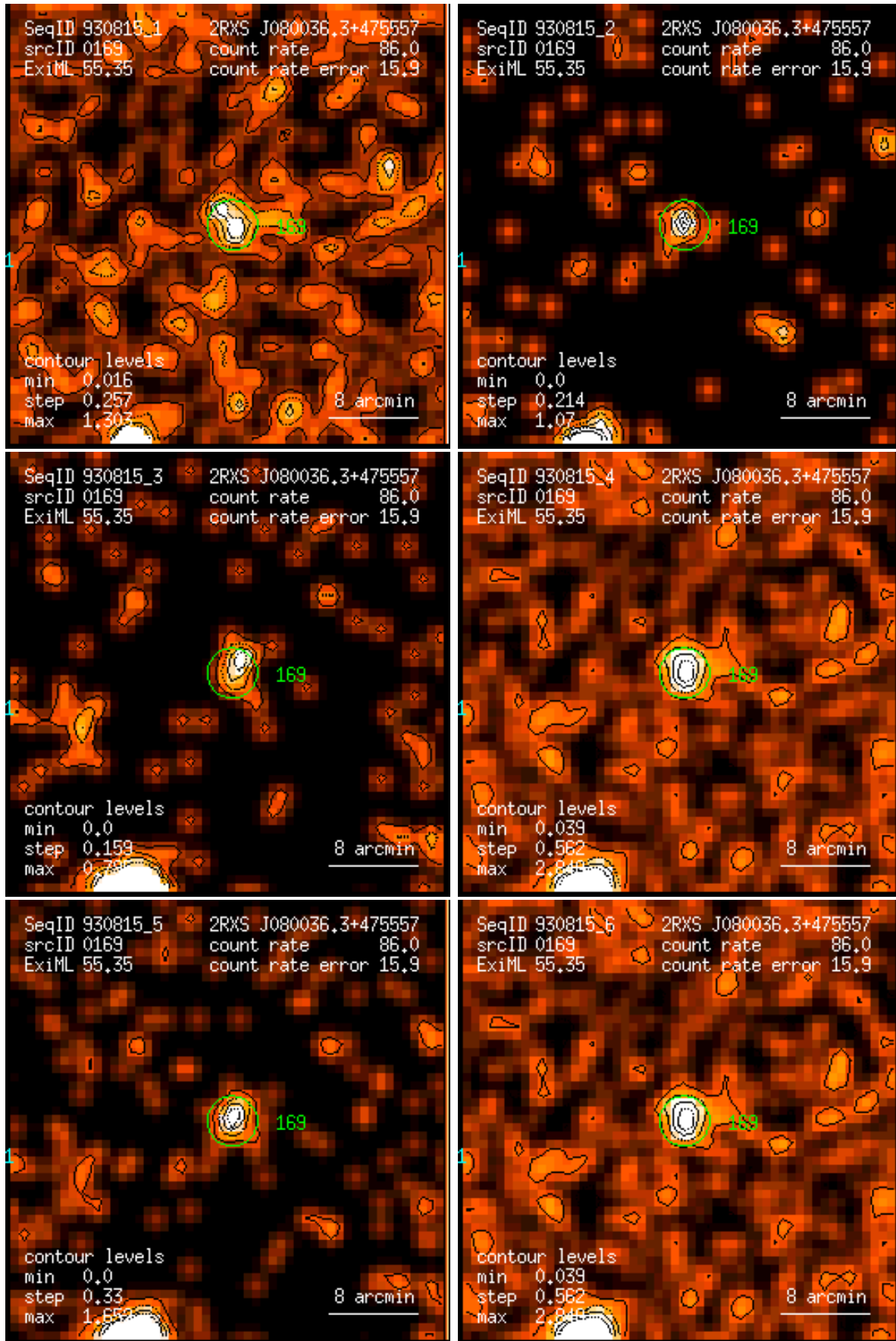
Figure 169: RASS 930815: detection 0169: band rate images, Gaussian filter: (1) PSPC channels 11 – 41, (2) 52 – 90, (3) 91 – 201, (4) 11 – 235, (5) 52 – 201, (6) 11 – 201. Broad band rates in counts/ks. Band rate contour levels in counts/ks/arcmin 2 .
