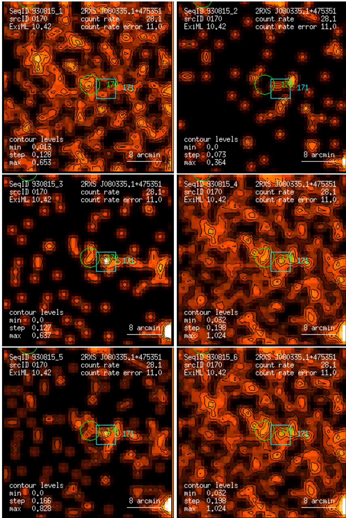
Figure 170: RASS 930815: detection 0170: band rate images, Gaussian filter: (1) PSPC channels 11 – 41, (2) 52 – 90, (3) 91 – 201, (4) 11 – 235, (5) 52 – 201, (6) 11 – 201. Broad band rates in counts/ks. Band rate contour levels in counts/ks/arcmin 2 .
