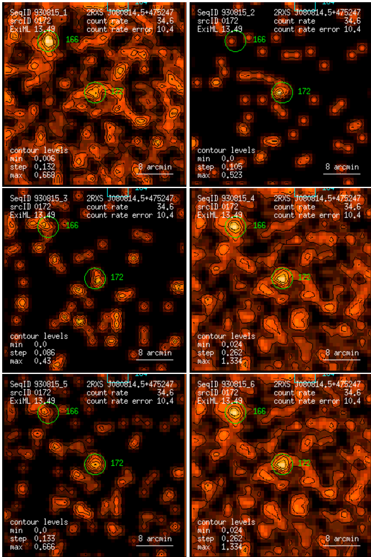
Figure 172: RASS 930815: detection 0172: band rate images, Gaussian filter: (1) PSPC channels 11 – 41, (2) 52 – 90, (3) 91 – 201, (4) 11 – 235, (5) 52 – 201, (6) 11 – 201. Broad band rates in counts/ks. Band rate contour levels in counts/ks/arcmin 2 .
