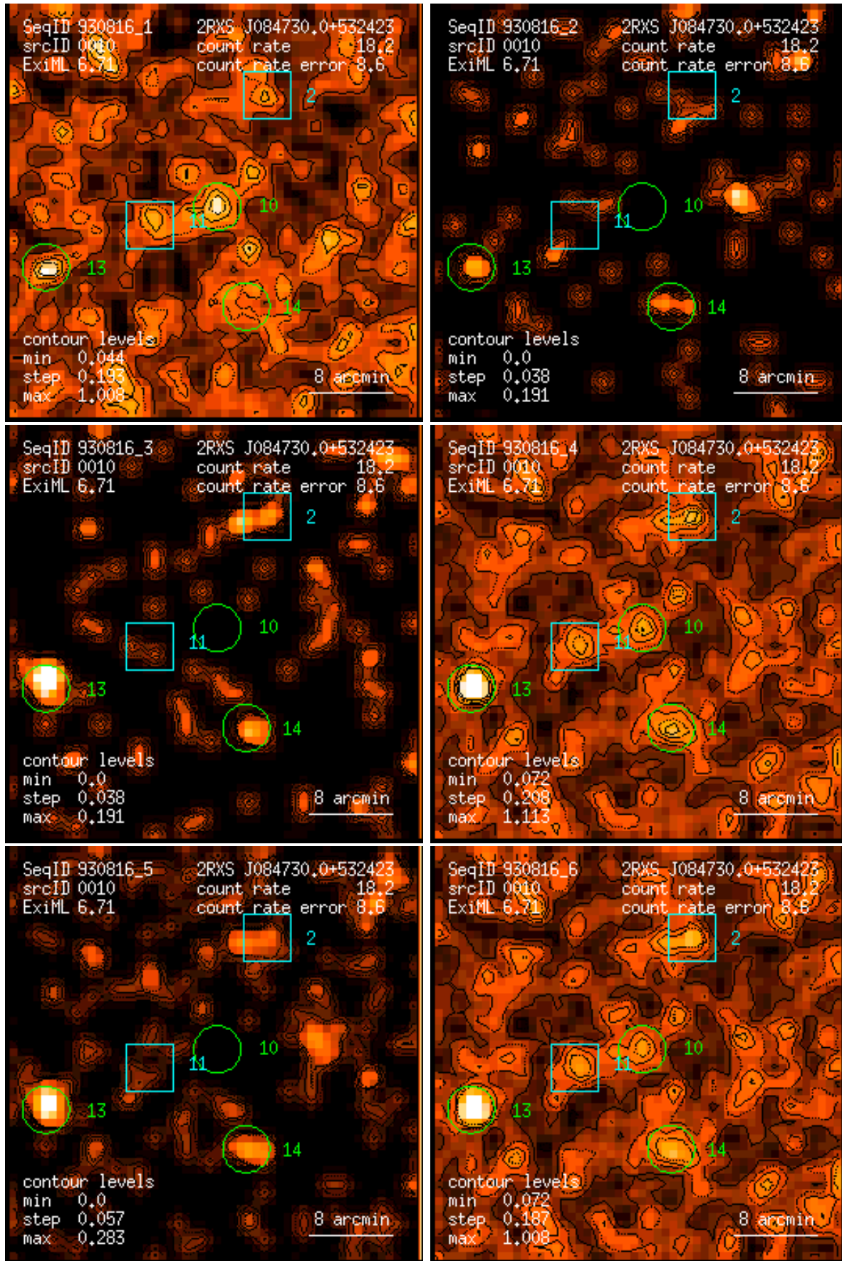
Figure 10: RASS 930816: detection 0010: band rate images, Gaussian filter: (1) PSPC channels 11 – 41, (2) 52 – 90, (3) 91 – 201, (4) 11 – 235, (5) 52 – 201, (6) 11 – 201. Broad band rates in counts/ks. Band rate contour levels in counts/ks/arcmin 2 .
