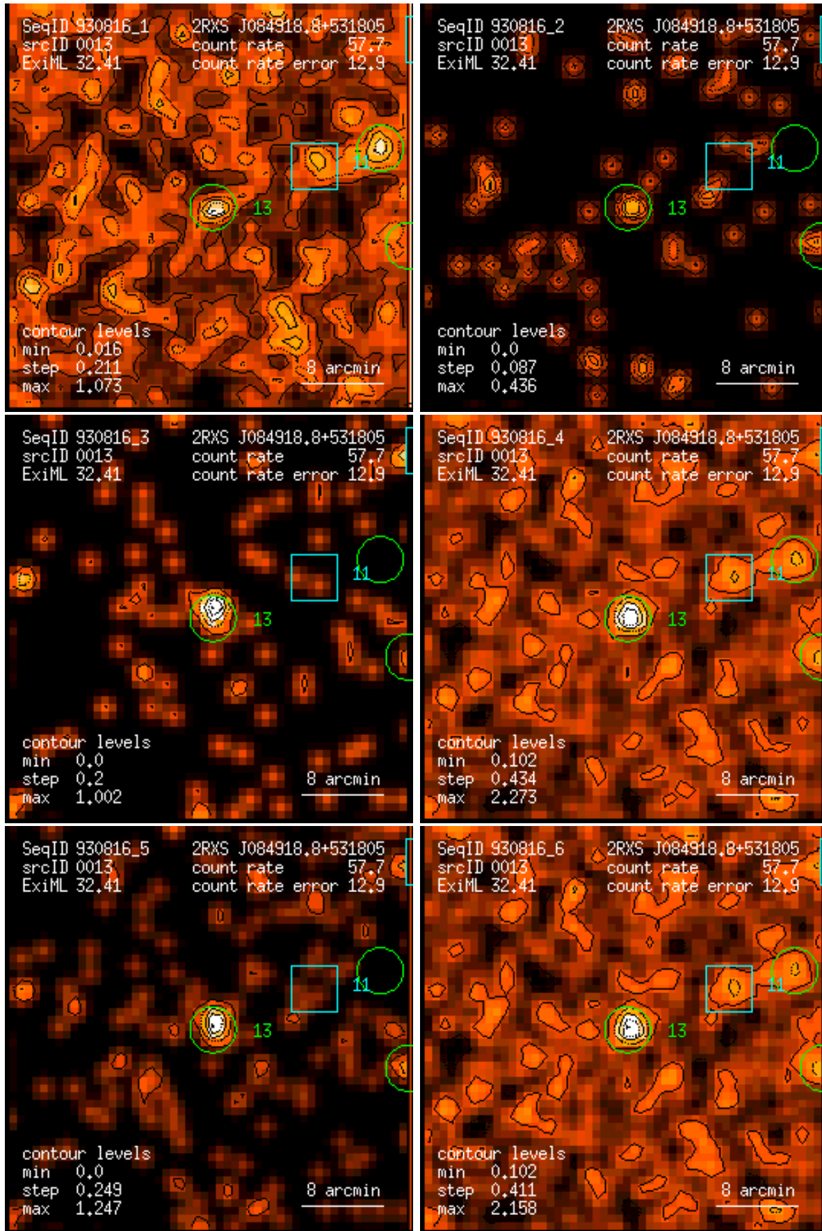
Figure 13: RASS 930816: detection 0013: band rate images, Gaussian filter: (1) PSPC channels 11 – 41, (2) 52 – 90, (3) 91 – 201, (4) 11 – 235, (5) 52 – 201, (6) 11 – 201. Broad band rates in counts/ks. Band rate contour levels in counts/ks/arcmin 2 .
