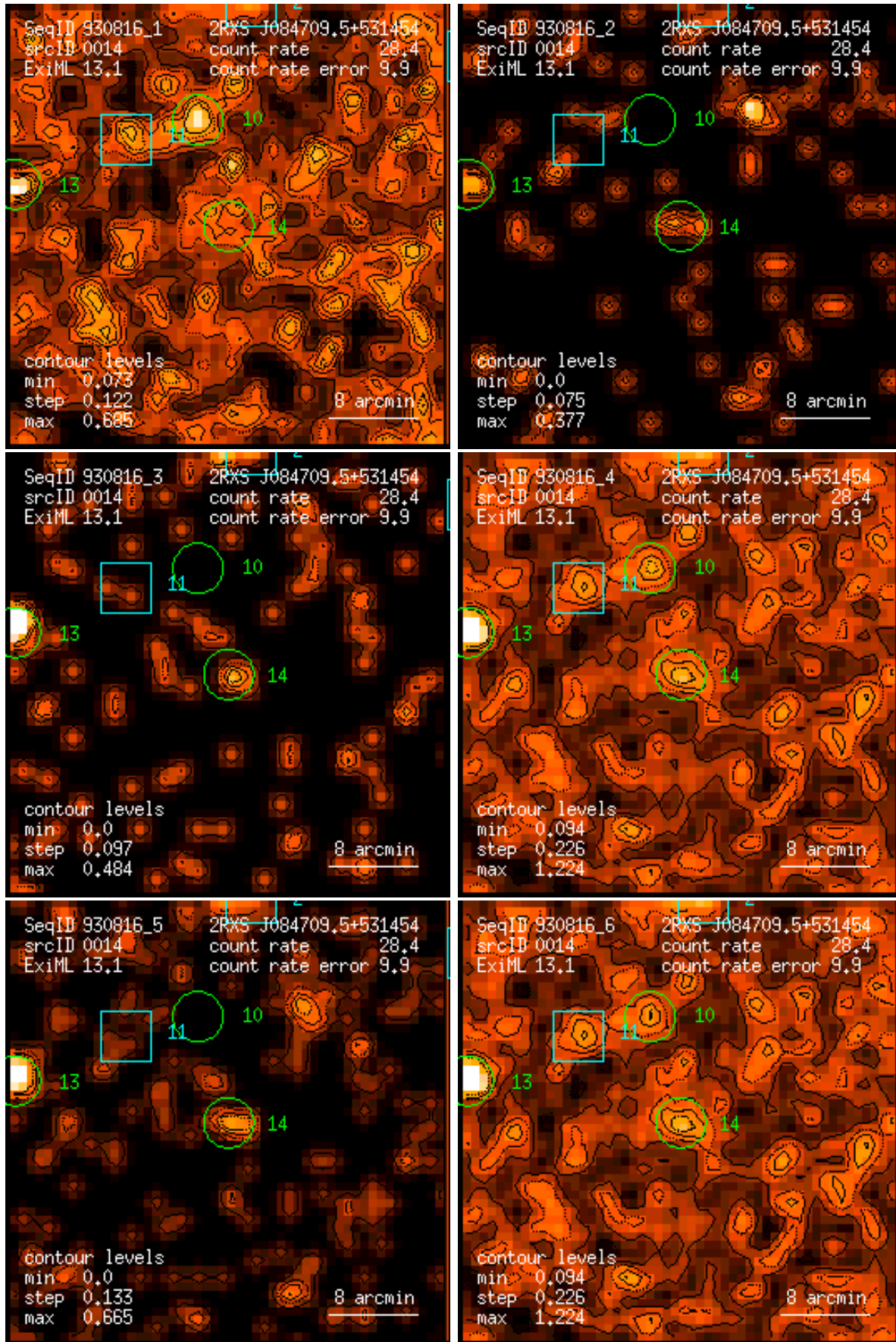
Figure 14: RASS 930816: detection 0014: band rate images, Gaussian filter: (1) PSPC channels 11 – 41, (2) 52 – 90, (3) 91 – 201, (4) 11 – 235, (5) 52 – 201, (6) 11 – 201. Broad band rates in counts/ks. Band rate contour levels in counts/ks/arcmin 2 .
