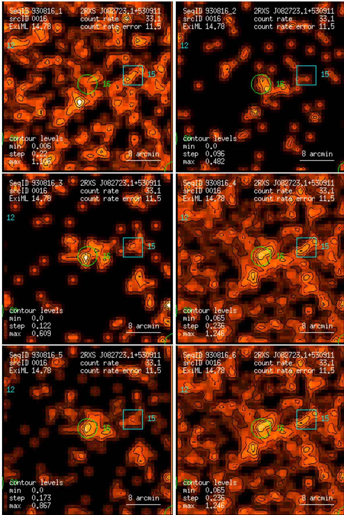
Figure 16: RASS 930816: detection 0016: band rate images, Gaussian filter: (1) PSPC channels 11 – 41, (2) 52 – 90, (3) 91 – 201, (4) 11 – 235, (5) 52 – 201, (6) 11 – 201. Broad band rates in counts/ks. Band rate contour levels in counts/ks/arcmin 2 .
