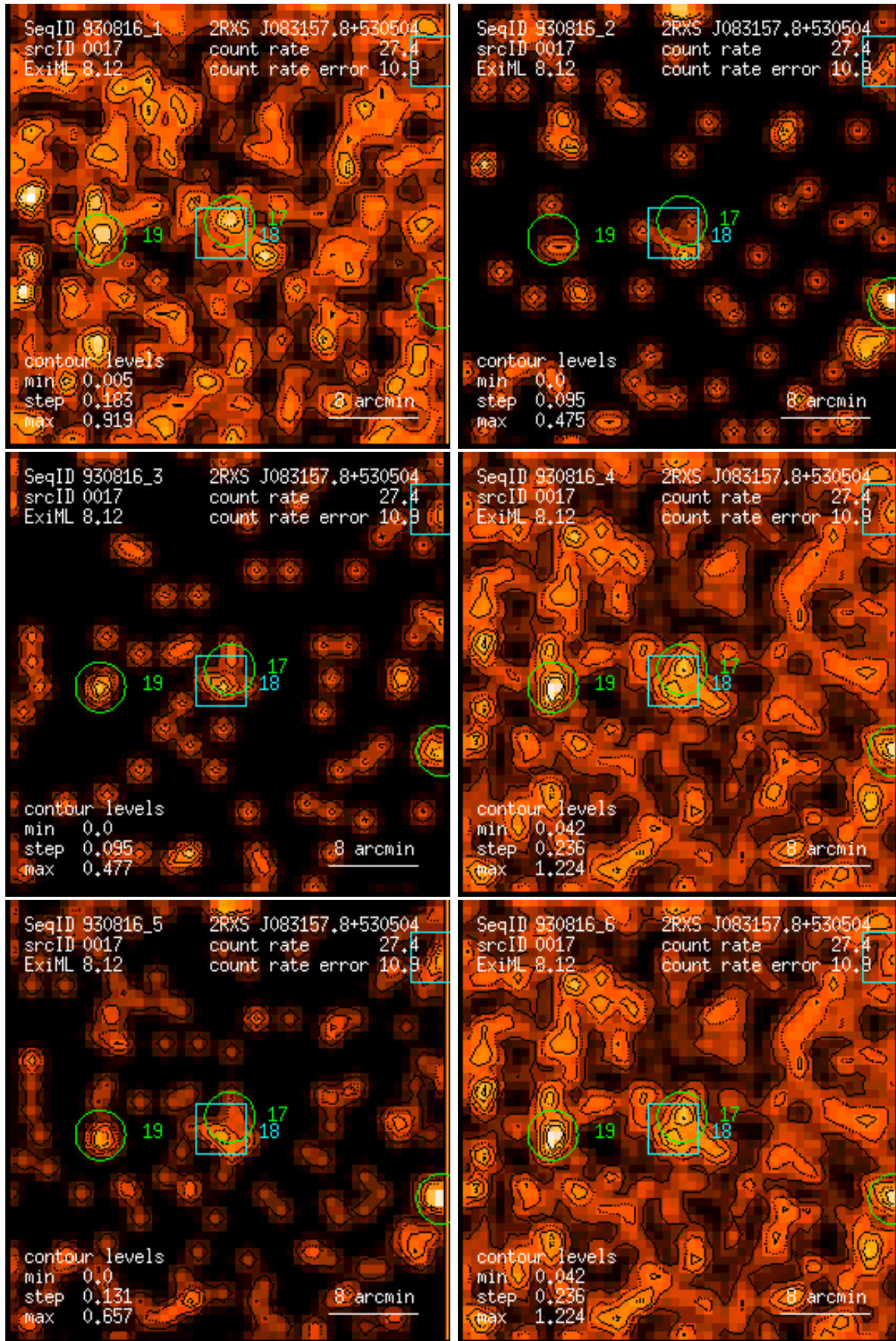
Figure 17: RASS 930816: detection 0017: band rate images, Gaussian filter: (1) PSPC channels 11 – 41, (2) 52 – 90, (3) 91 – 201, (4) 11 – 235, (5) 52 – 201, (6) 11 – 201. Broad band rates in counts/ks. Band rate contour levels in counts/ks/arcmin 2 .
