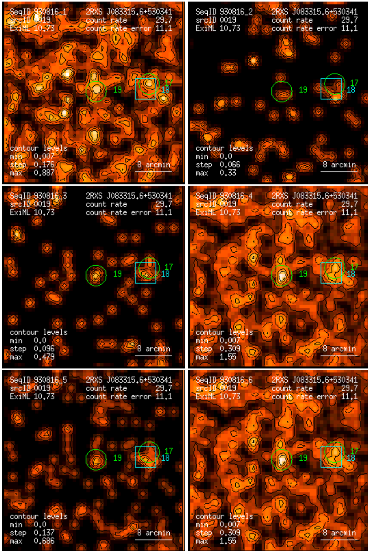
Figure 19: RASS 930816: detection 0019: band rate images, Gaussian filter: (1) PSPC channels 11 – 41, (2) 52 – 90, (3) 91 – 201, (4) 11 – 235, (5) 52 – 201, (6) 11 – 201. Broad band rates in counts/ks. Band rate contour levels in counts/ks/arcmin 2 .
