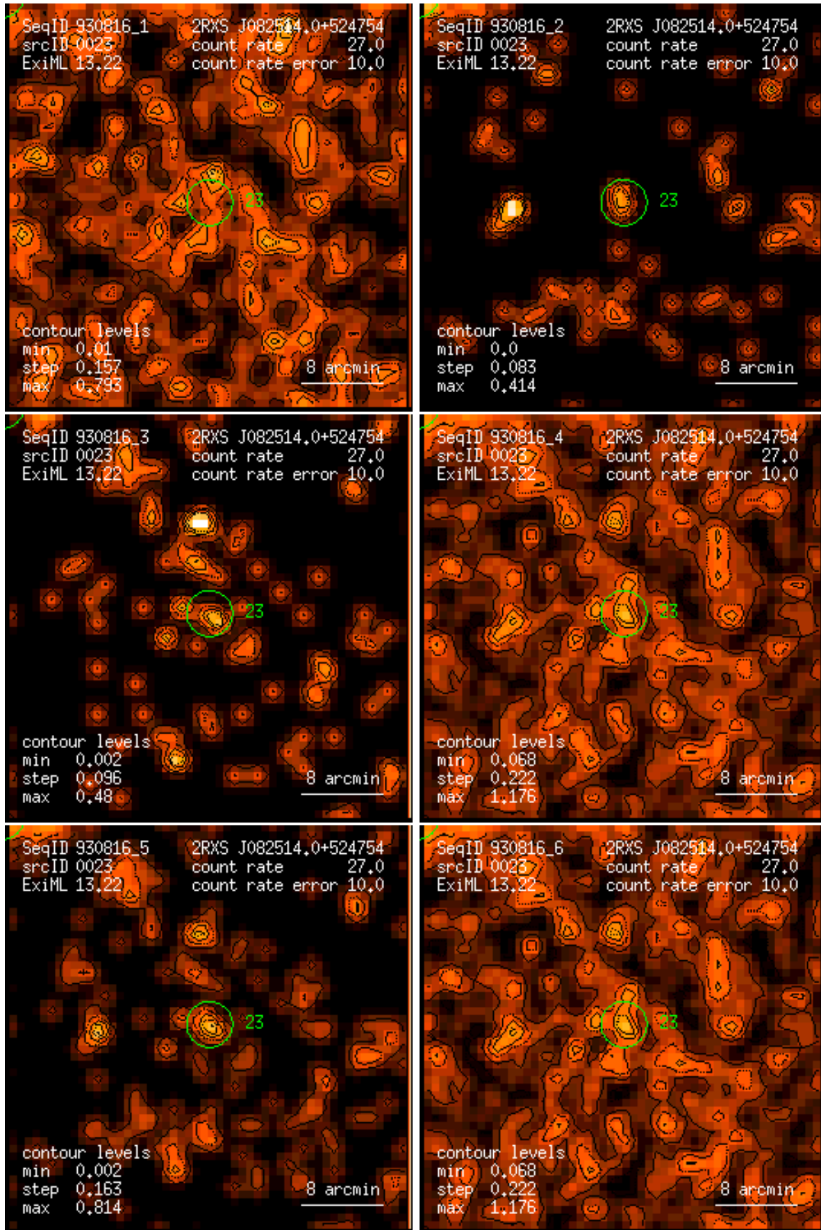
Figure 23: RASS 930816: detection 0023: band rate images, Gaussian filter: (1) PSPC channels 11 – 41, (2) 52 – 90, (3) 91 – 201, (4) 11 – 235, (5) 52 – 201, (6) 11 – 201. Broad band rates in counts/ks. Band rate contour levels in counts/ks/arcmin 2 .
