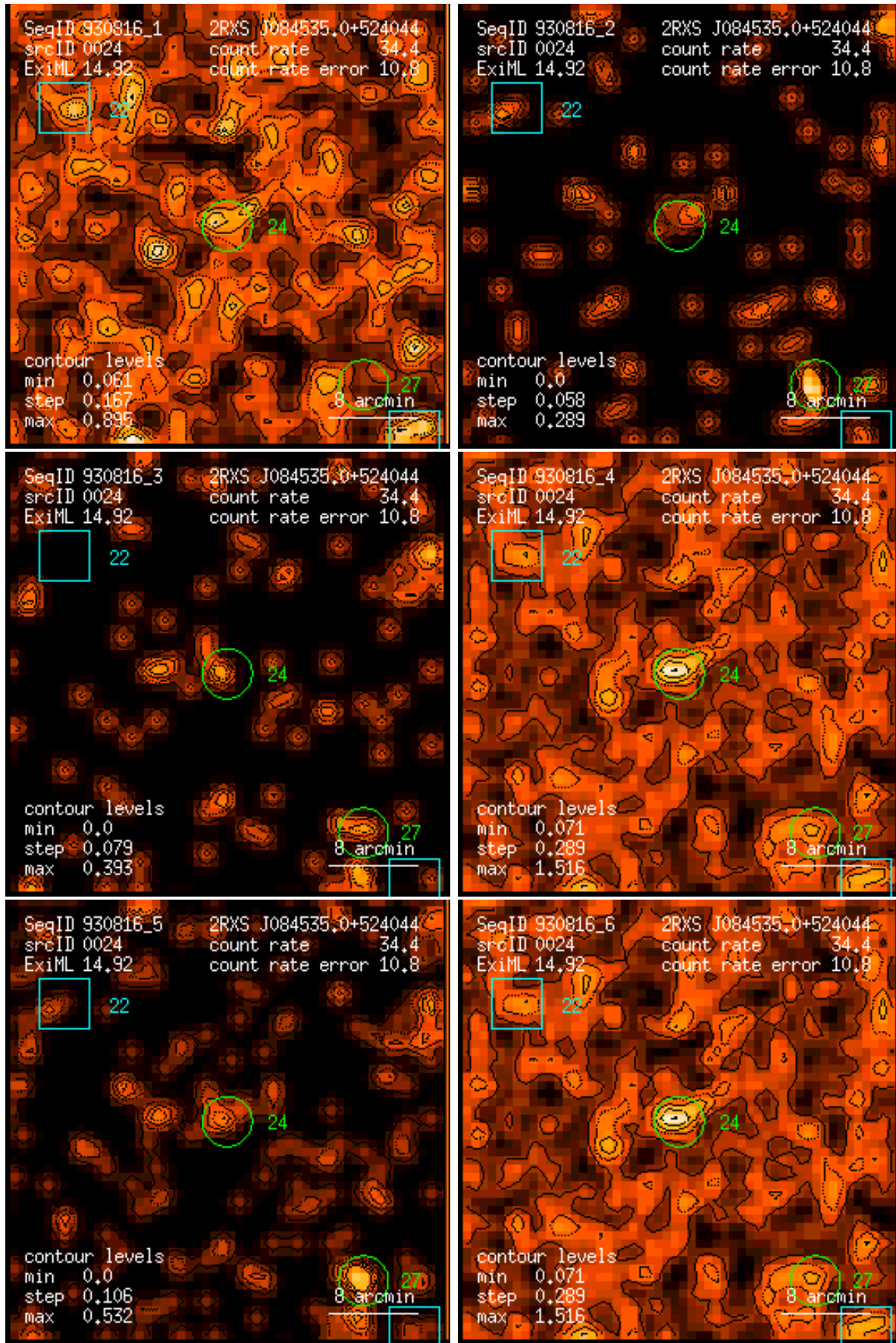
Figure 24: RASS 930816: detection 0024: band rate images, Gaussian filter: (1) PSPC channels 11 – 41, (2) 52 – 90, (3) 91 – 201, (4) 11 – 235, (5) 52 – 201, (6) 11 – 201. Broad band rates in counts/ks. Band rate contour levels in counts/ks/arcmin 2 .
