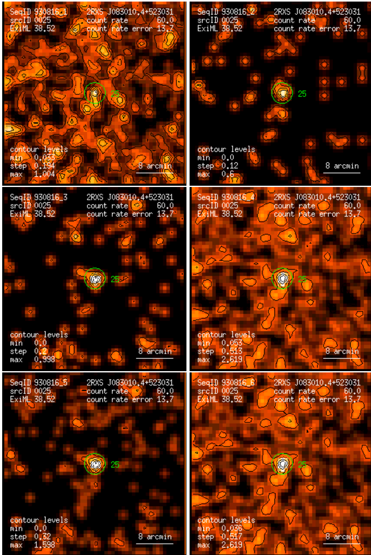
Figure 25: RASS 930816: detection 0025: band rate images, Gaussian filter: (1) PSPC channels 11 – 41, (2) 52 – 90, (3) 91 – 201, (4) 11 – 235, (5) 52 – 201, (6) 11 – 201. Broad band rates in counts/ks. Band rate contour levels in counts/ks/arcmin 2 .
