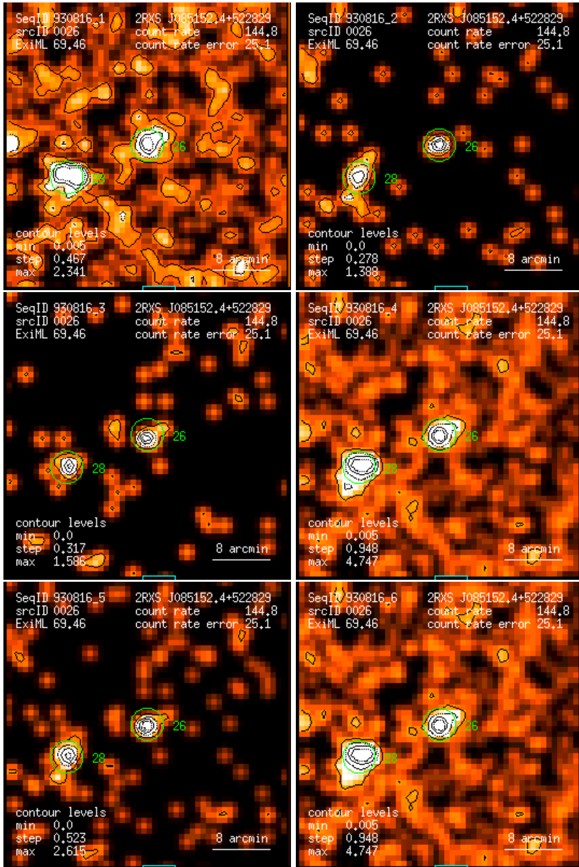
Figure 26: RASS 930816: detection 0026: band rate images, Gaussian filter: (1) PSPC channels 11 – 41, (2) 52 – 90, (3) 91 – 201, (4) 11 – 235, (5) 52 – 201, (6) 11 – 201. Broad band rates in counts/ks. Band rate contour levels in counts/ks/arcmin 2 .
