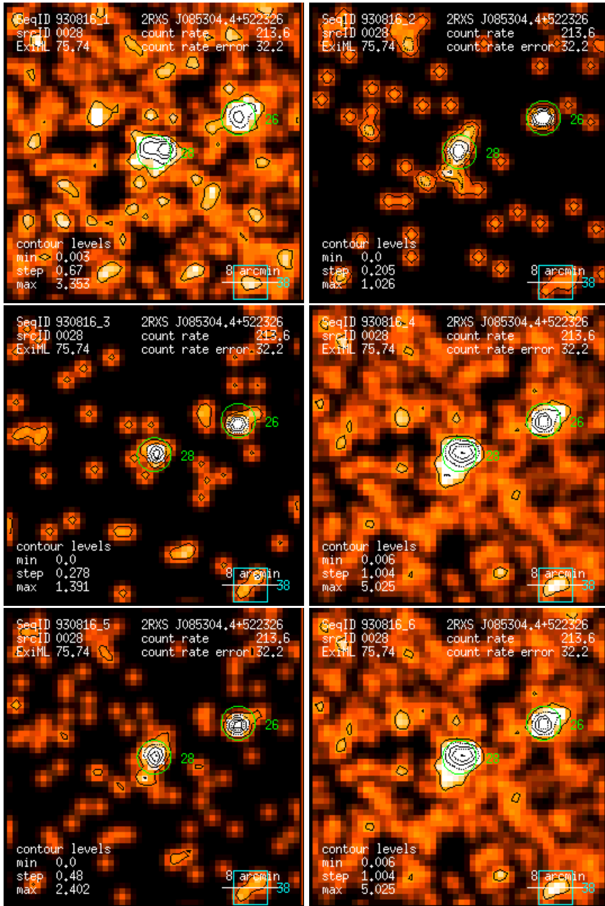
Figure 28: RASS 930816: detection 0028: band rate images, Gaussian filter: (1) PSPC channels 11 – 41, (2) 52 – 90, (3) 91 – 201, (4) 11 – 235, (5) 52 – 201, (6) 11 – 201. Broad band rates in counts/ks. Band rate contour levels in counts/ks/arcmin 2 .
