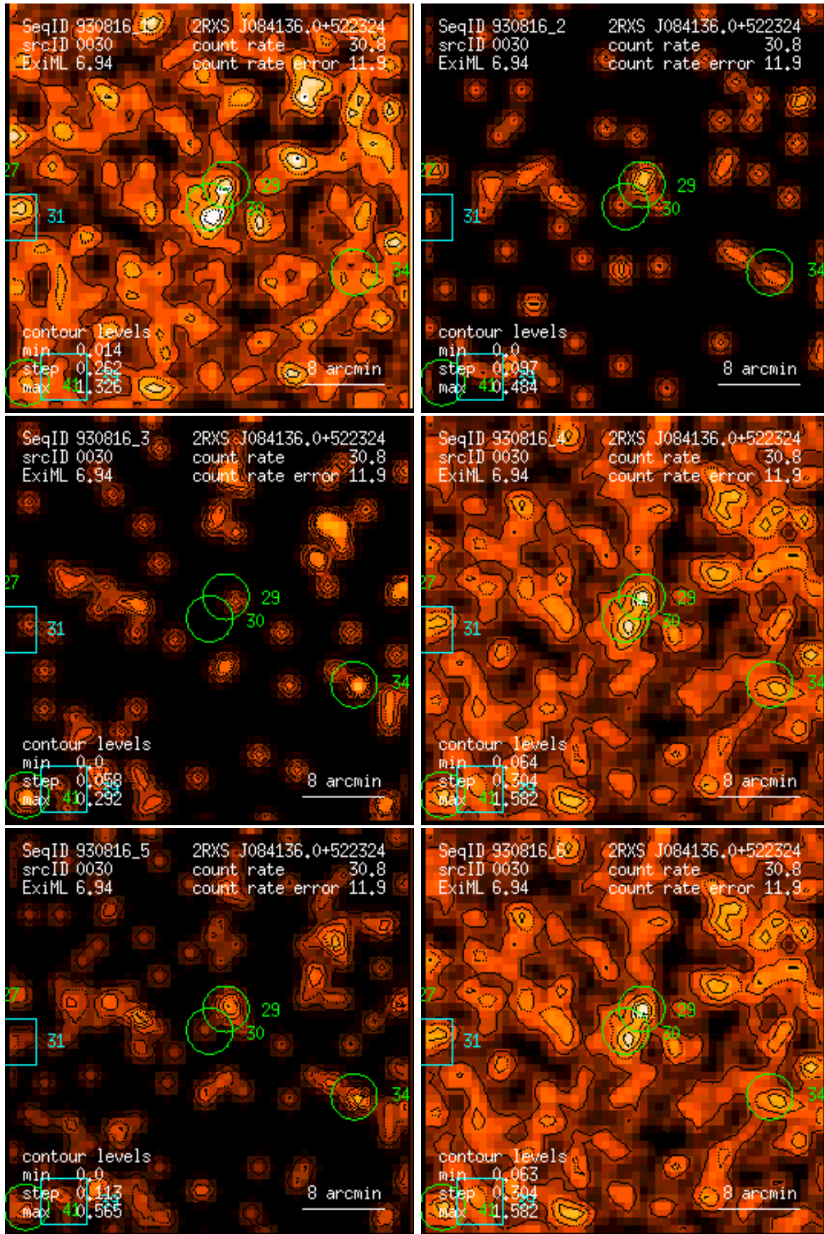
Figure 30: RASS 930816: detection 0030: band rate images, Gaussian filter: (1) PSPC channels 11 – 41, (2) 52 – 90, (3) 91 – 201, (4) 11 – 235, (5) 52 – 201, (6) 11 – 201. Broad band rates in counts/ks. Band rate contour levels in counts/ks/arcmin 2 .
