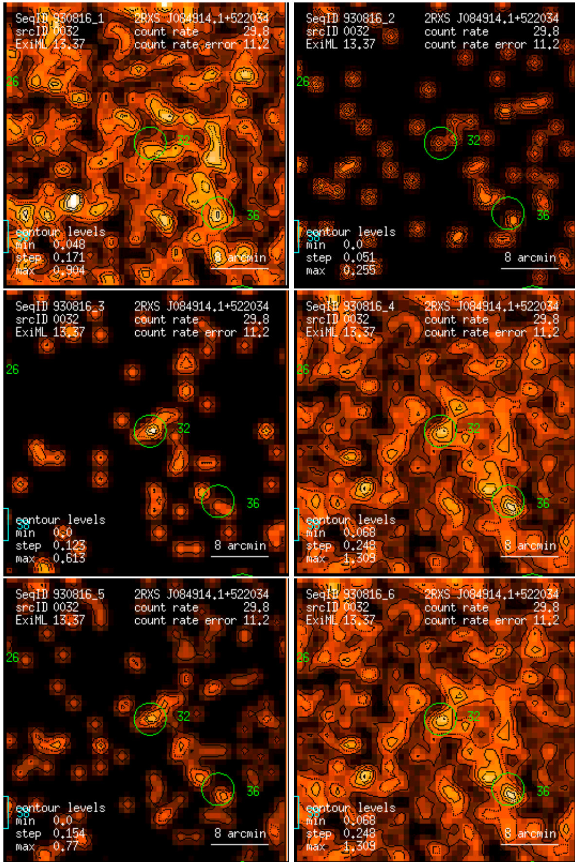
Figure 32: RASS 930816: detection 0032: band rate images, Gaussian filter: (1) PSPC channels 11 – 41, (2) 52 – 90, (3) 91 – 201, (4) 11 – 235, (5) 52 – 201, (6) 11 – 201. Broad band rates in counts/ks. Band rate contour levels in counts/ks/arcmin 2 .
