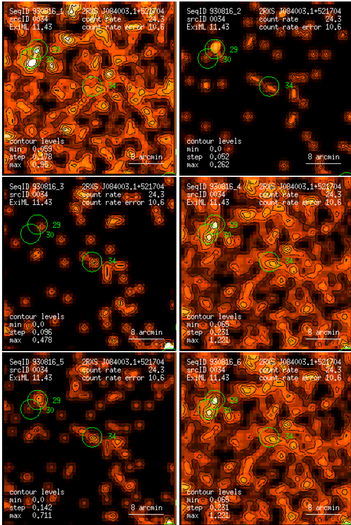
Figure 34: RASS 930816: detection 0034: band rate images, Gaussian filter: (1) PSPC channels 11 – 41, (2) 52 – 90, (3) 91 – 201, (4) 11 – 235, (5) 52 – 201, (6) 11 – 201. Broad band rates in counts/ks. Band rate contour levels in counts/ks/arcmin 2 .
