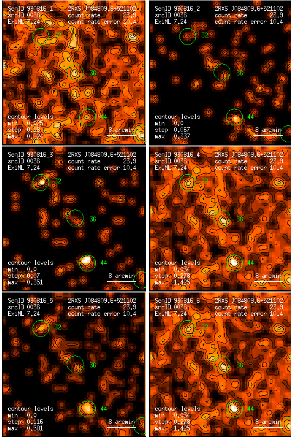
Figure 36: RASS 930816: detection 0036: band rate images, Gaussian filter: (1) PSPC channels 11 – 41, (2) 52 – 90, (3) 91 – 201, (4) 11 – 235, (5) 52 – 201, (6) 11 – 201. Broad band rates in counts/ks. Band rate contour levels in counts/ks/arcmin 2 .
