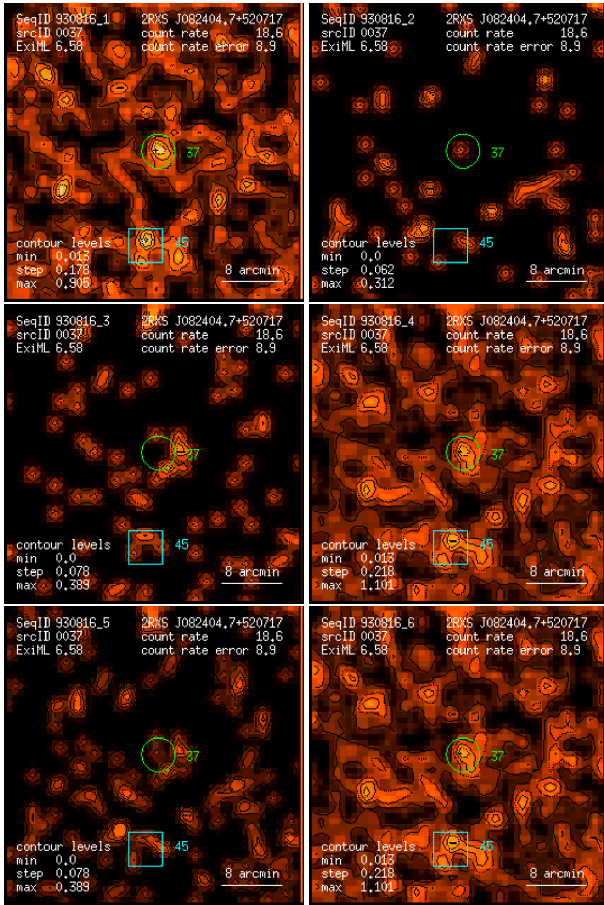
Figure 37: RASS 930816: detection 0037: band rate images, Gaussian filter: (1) PSPC channels 11 – 41, (2) 52 – 90, (3) 91 – 201, (4) 11 – 235, (5) 52 – 201, (6) 11 – 201. Broad band rates in counts/ks. Band rate contour levels in counts/ks/arcmin 2 .
