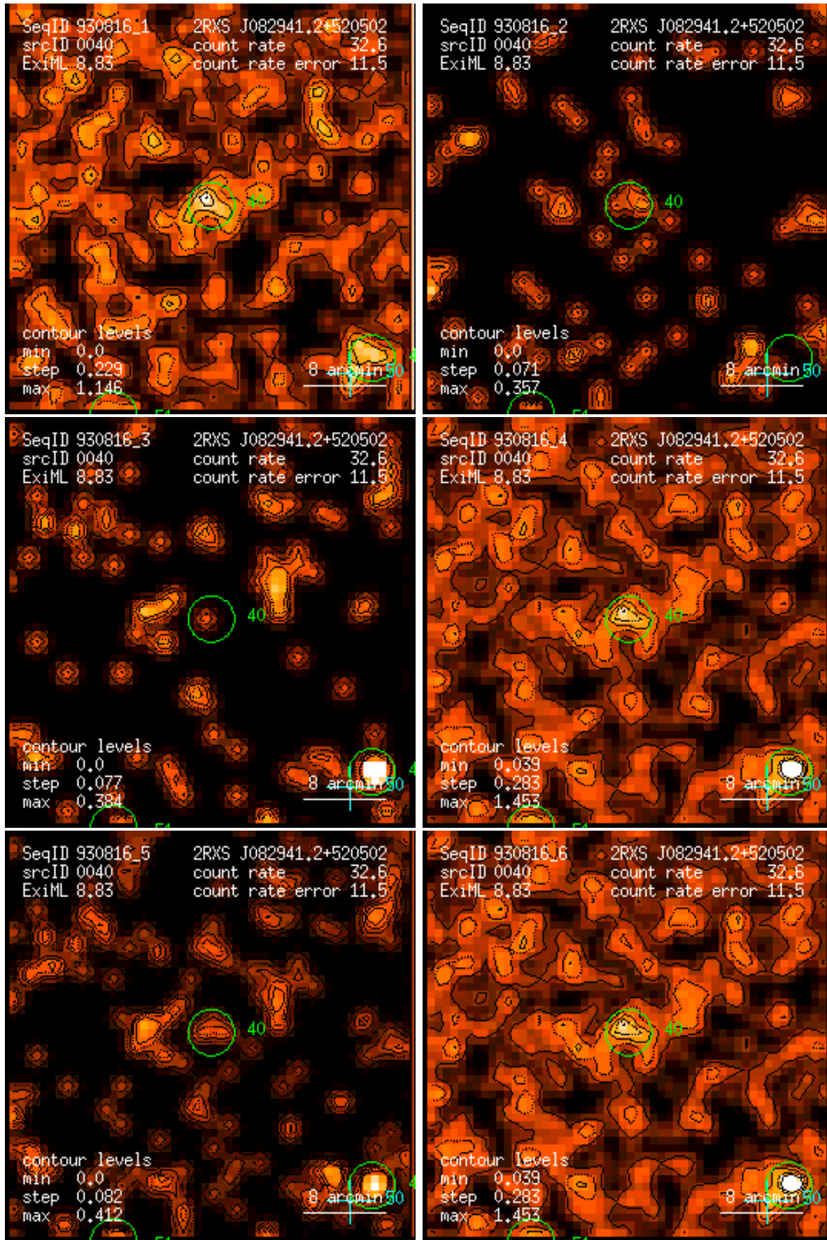
Figure 40: RASS 930816: detection 0040: band rate images, Gaussian filter: (1) PSPC channels 11 – 41, (2) 52 – 90, (3) 91 – 201, (4) 11 – 235, (5) 52 – 201, (6) 11 – 201. Broad band rates in counts/ks. Band rate contour levels in counts/ks/arcmin 2 .
