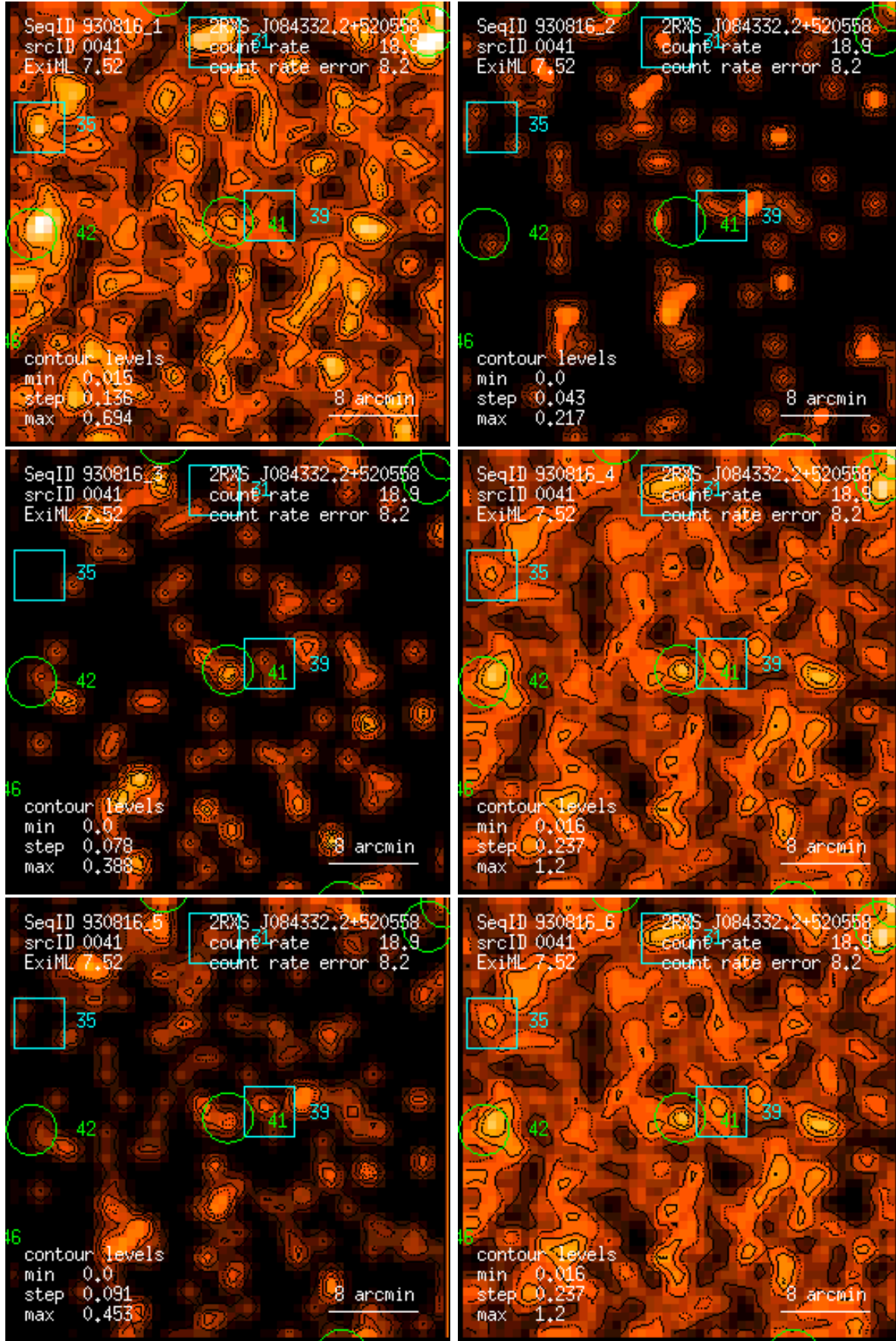
Figure 41: RASS 930816: detection 0041: band rate images, Gaussian filter: (1) PSPC channels 11 – 41, (2) 52 – 90, (3) 91 – 201, (4) 11 – 235, (5) 52 – 201, (6) 11 – 201. Broad band rates in counts/ks. Band rate contour levels in counts/ks/arcmin 2 .
