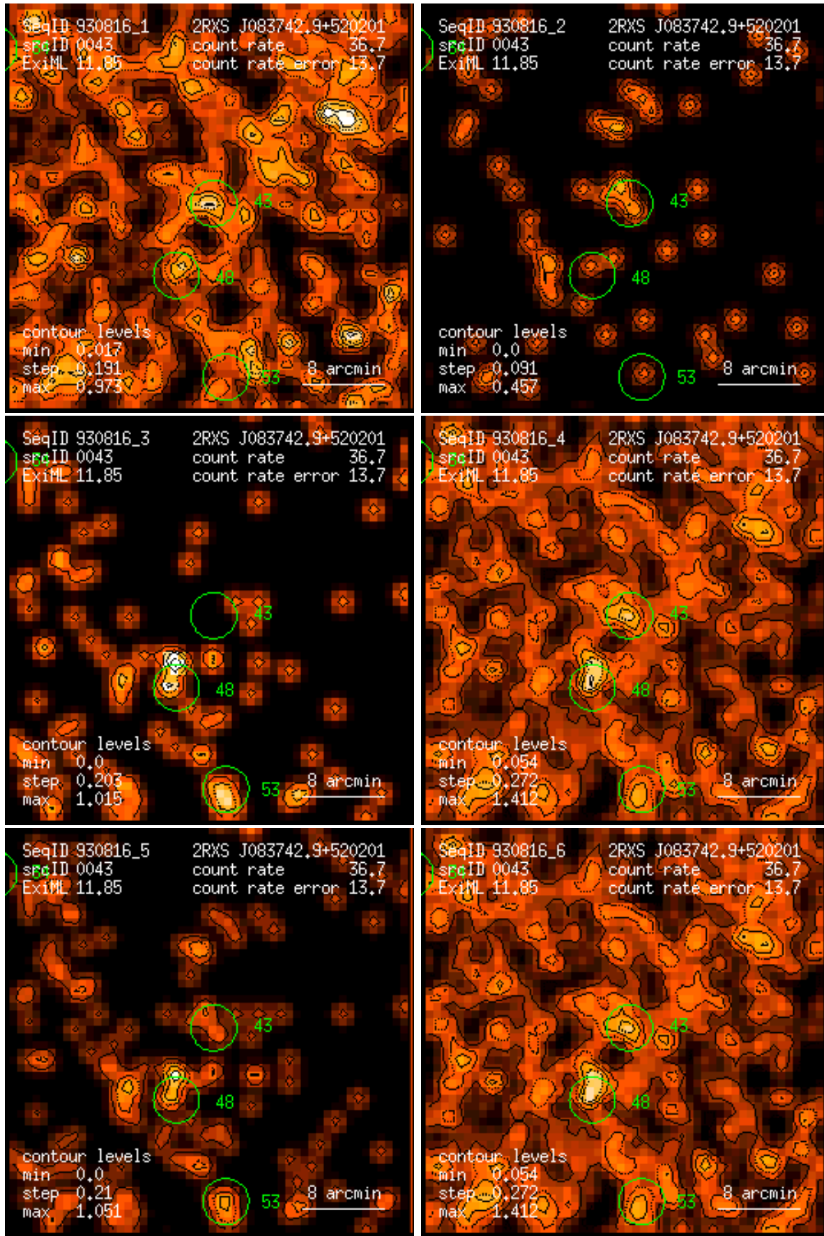
Figure 43: RASS 930816: detection 0043: band rate images, Gaussian filter: (1) PSPC channels 11 – 41, (2) 52 – 90, (3) 91 – 201, (4) 11 – 235, (5) 52 – 201, (6) 11 – 201. Broad band rates in counts/ks. Band rate contour levels in counts/ks/arcmin 2 .
