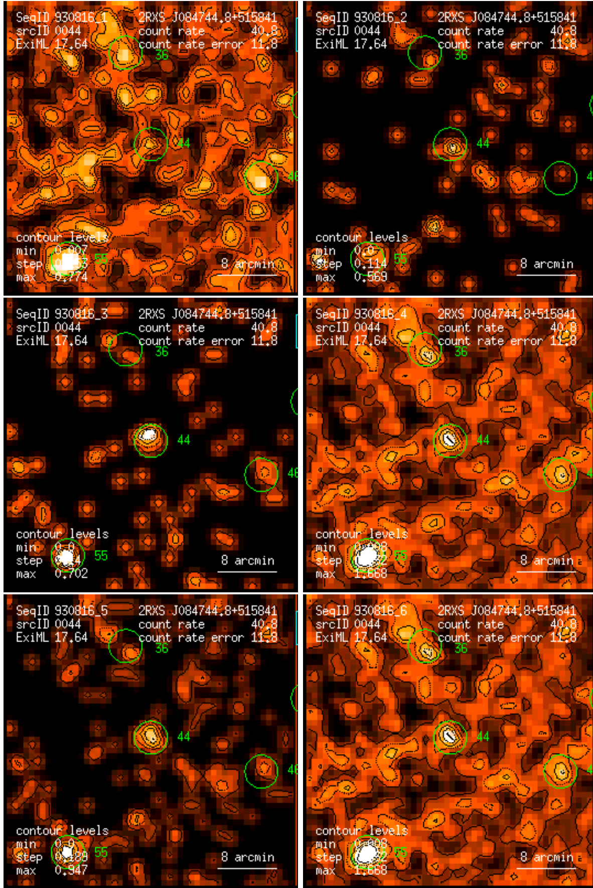
Figure 44: RASS 930816: detection 0044: band rate images, Gaussian filter: (1) PSPC channels 11 – 41, (2) 52 – 90, (3) 91 – 201, (4) 11 – 235, (5) 52 – 201, (6) 11 – 201. Broad band rates in counts/ks. Band rate contour levels in counts/ks/arcmin 2 .
