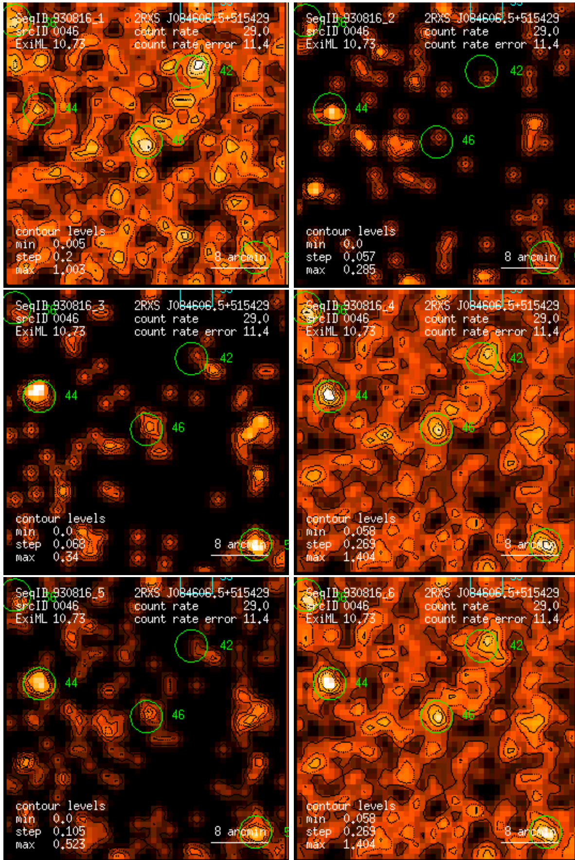
Figure 46: RASS 930816: detection 0046: band rate images, Gaussian filter: (1) PSPC channels 11 – 41, (2) 52 – 90, (3) 91 – 201, (4) 11 – 235, (5) 52 – 201, (6) 11 – 201. Broad band rates in counts/ks. Band rate contour levels in counts/ks/arcmin 2 .
