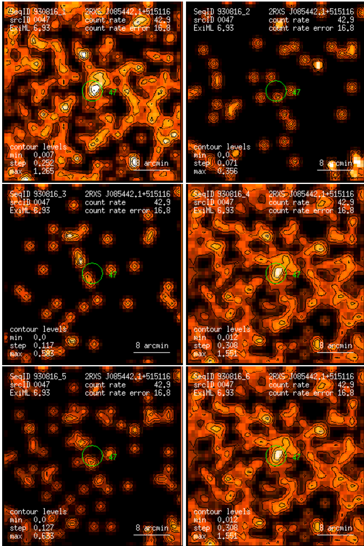
Figure 47: RASS 930816: detection 0047: band rate images, Gaussian filter: (1) PSPC channels 11 – 41, (2) 52 – 90, (3) 91 – 201, (4) 11 – 235, (5) 52 – 201, (6) 11 – 201. Broad band rates in counts/ks. Band rate contour levels in counts/ks/arcmin 2 .
