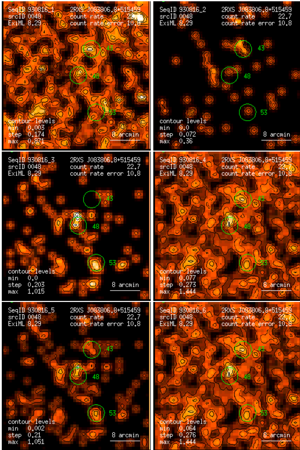
Figure 48: RASS 930816: detection 0048: band rate images, Gaussian filter: (1) PSPC channels 11 – 41, (2) 52 – 90, (3) 91 – 201, (4) 11 – 235, (5) 52 – 201, (6) 11 – 201. Broad band rates in counts/ks. Band rate contour levels in counts/ks/arcmin 2 .
