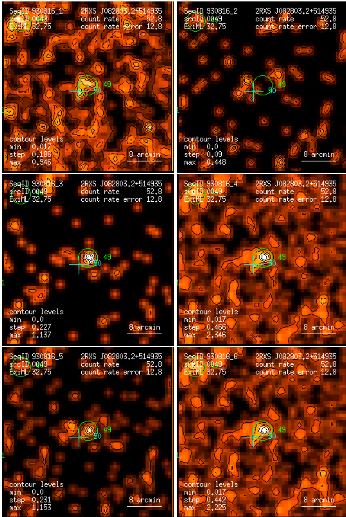
Figure 49: RASS 930816: detection 0049: band rate images, Gaussian filter: (1) PSPC channels 11 – 41, (2) 52 – 90, (3) 91 – 201, (4) 11 – 235, (5) 52 – 201, (6) 11 – 201. Broad band rates in counts/ks. Band rate contour levels in counts/ks/arcmin 2 .
