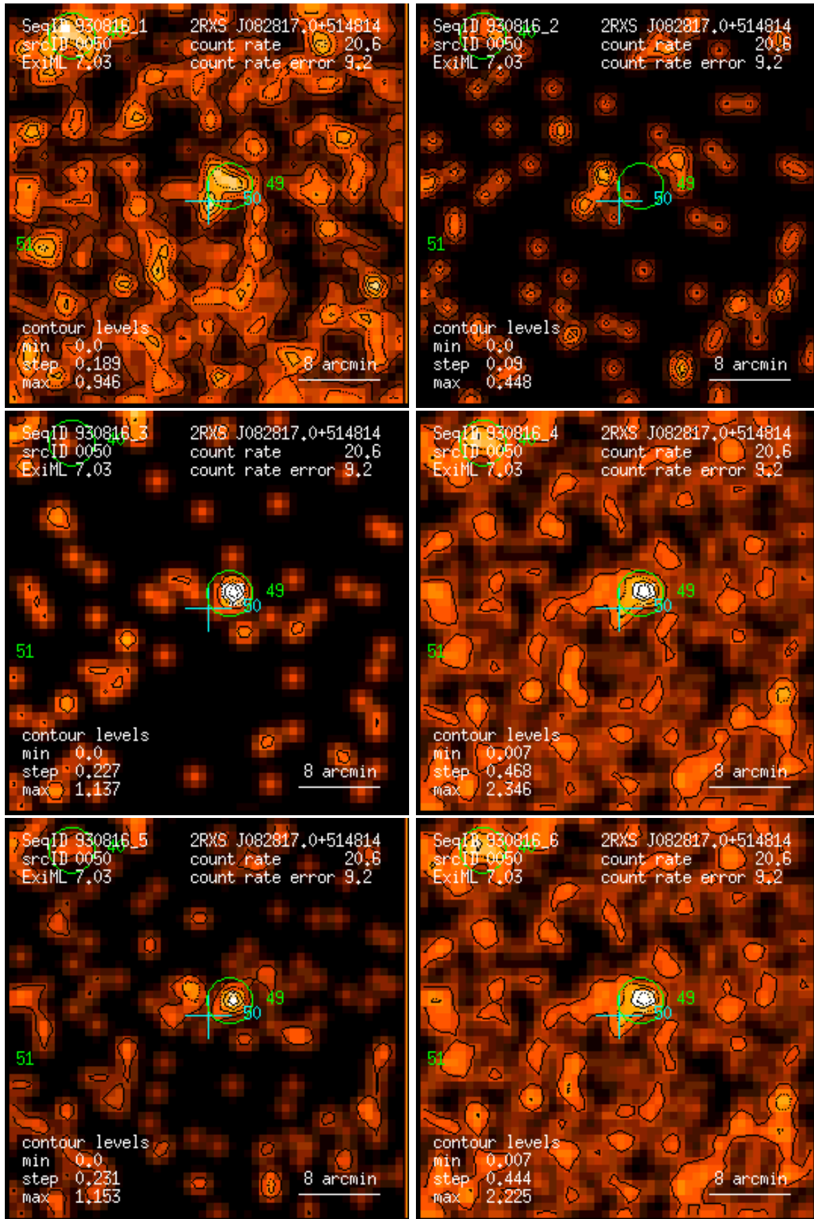
Figure 50: RASS 930816: detection 0050: band rate images, Gaussian filter: (1) PSPC channels 11 – 41, (2) 52 – 90, (3) 91 – 201, (4) 11 – 235, (5) 52 – 201, (6) 11 – 201. Broad band rates in counts/ks. Band rate contour levels in counts/ks/arcmin 2 .
