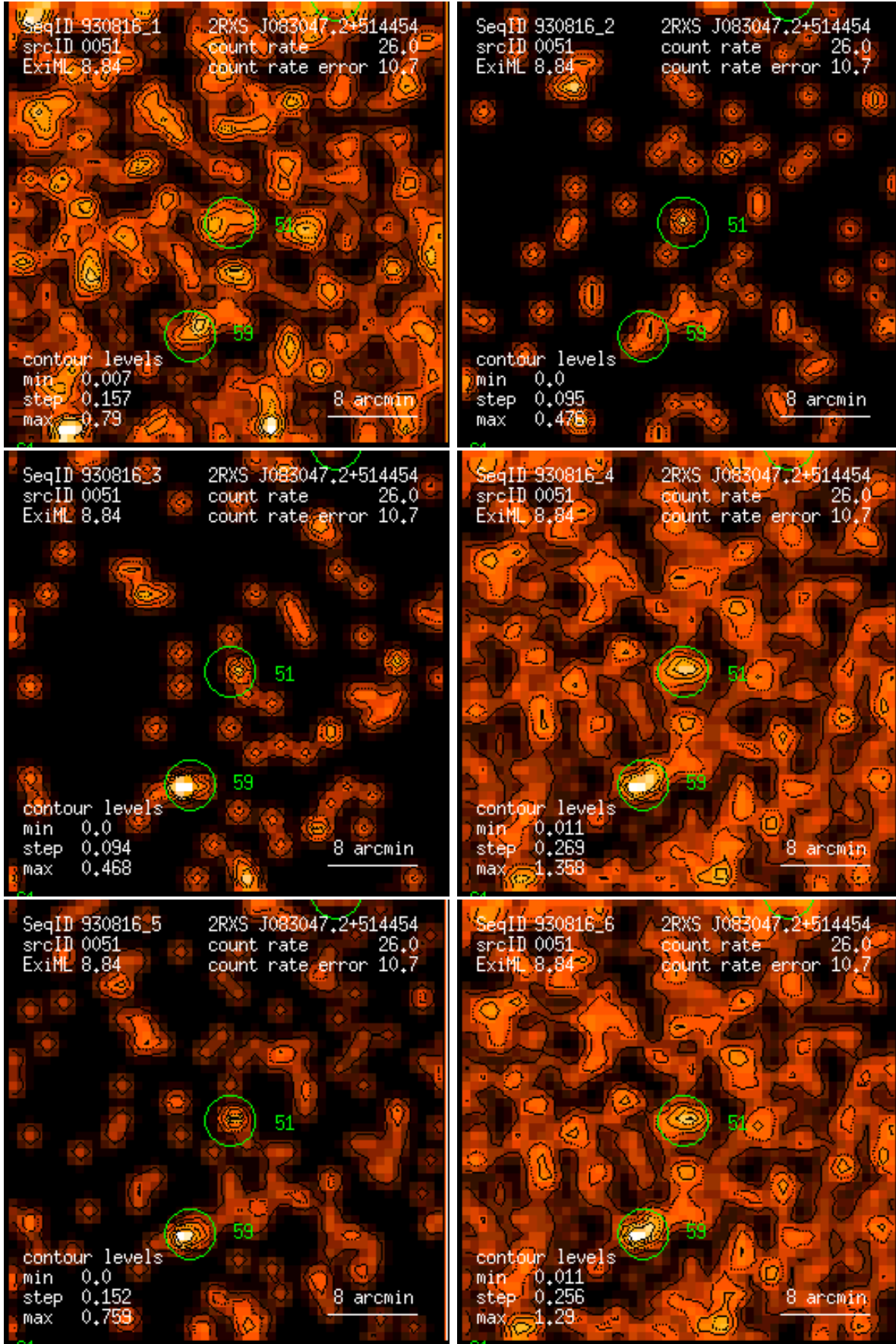
Figure 51: RASS 930816: detection 0051: band rate images, Gaussian filter: (1) PSPC channels 11 – 41, (2) 52 – 90, (3) 91 – 201, (4) 11 – 235, (5) 52 – 201, (6) 11 – 201. Broad band rates in counts/ks. Band rate contour levels in counts/ks/arcmin 2 .
