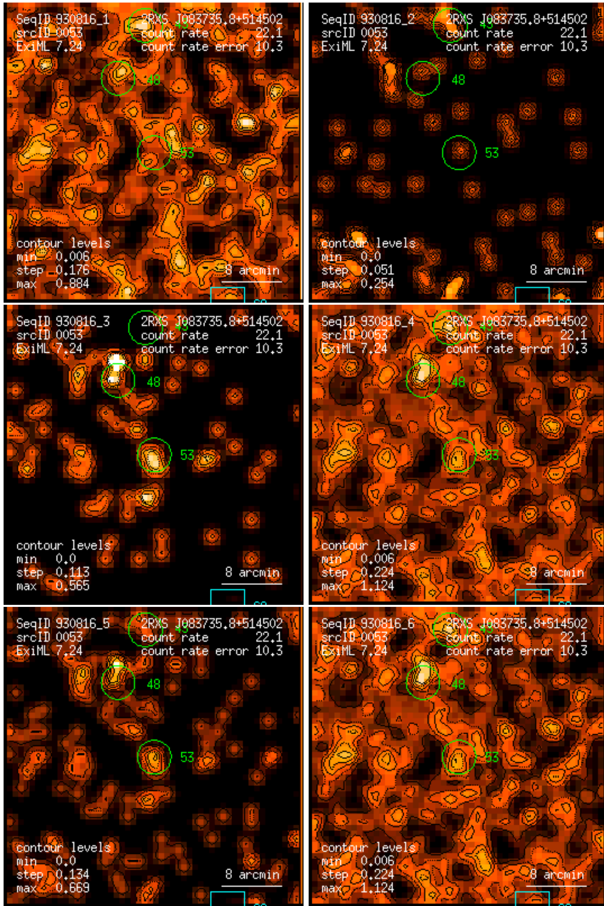
Figure 53: RASS 930816: detection 0053: band rate images, Gaussian filter: (1) PSPC channels 11 – 41, (2) 52 – 90, (3) 91 – 201, (4) 11 – 235, (5) 52 – 201, (6) 11 – 201. Broad band rates in counts/ks. Band rate contour levels in counts/ks/arcmin 2 .
