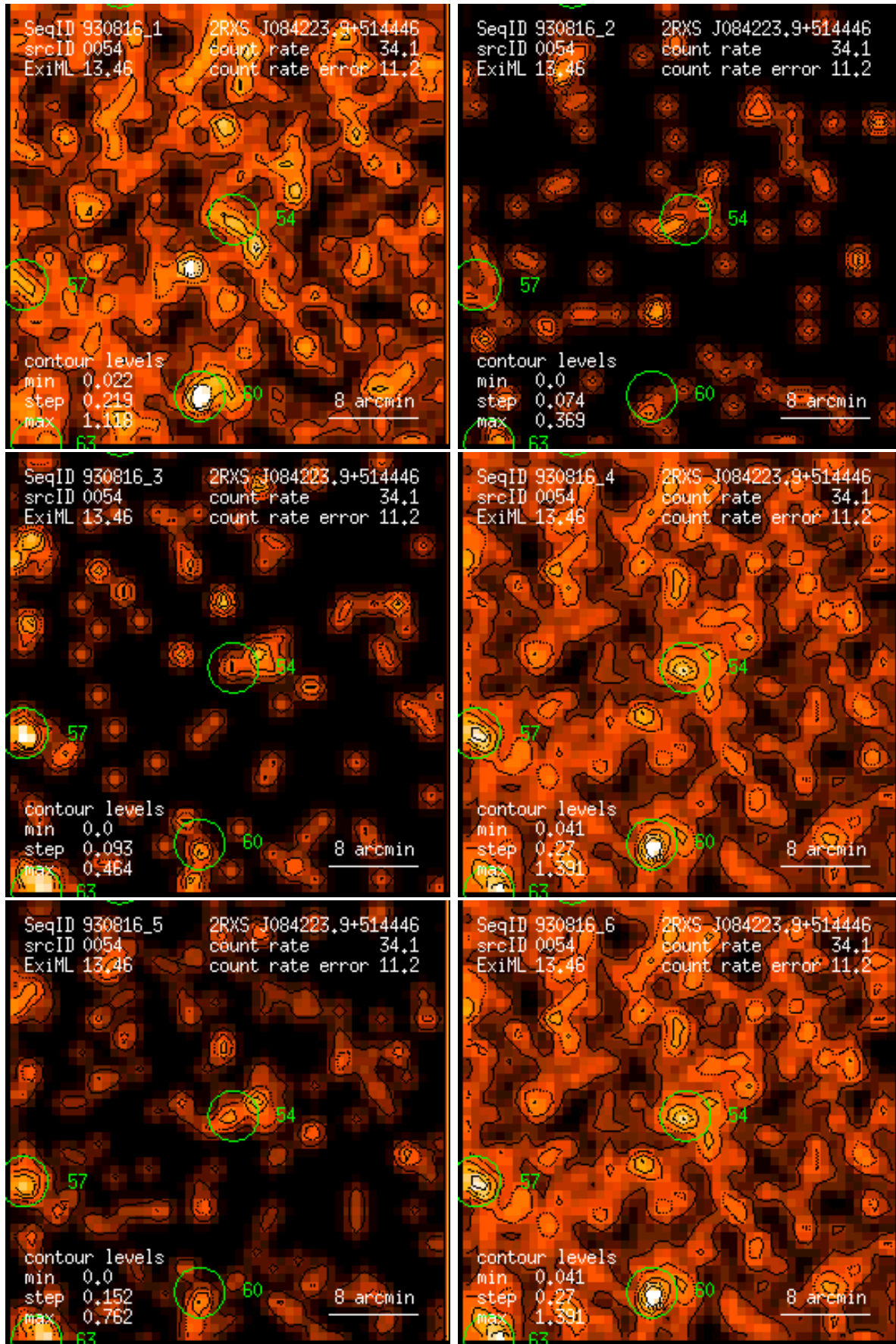
Figure 54: RASS 930816: detection 0054: band rate images, Gaussian filter: (1) PSPC channels 11 – 41, (2) 52 – 90, (3) 91 – 201, (4) 11 – 235, (5) 52 – 201, (6) 11 – 201. Broad band rates in counts/ks. Band rate contour levels in counts/ks/arcmin 2 .
