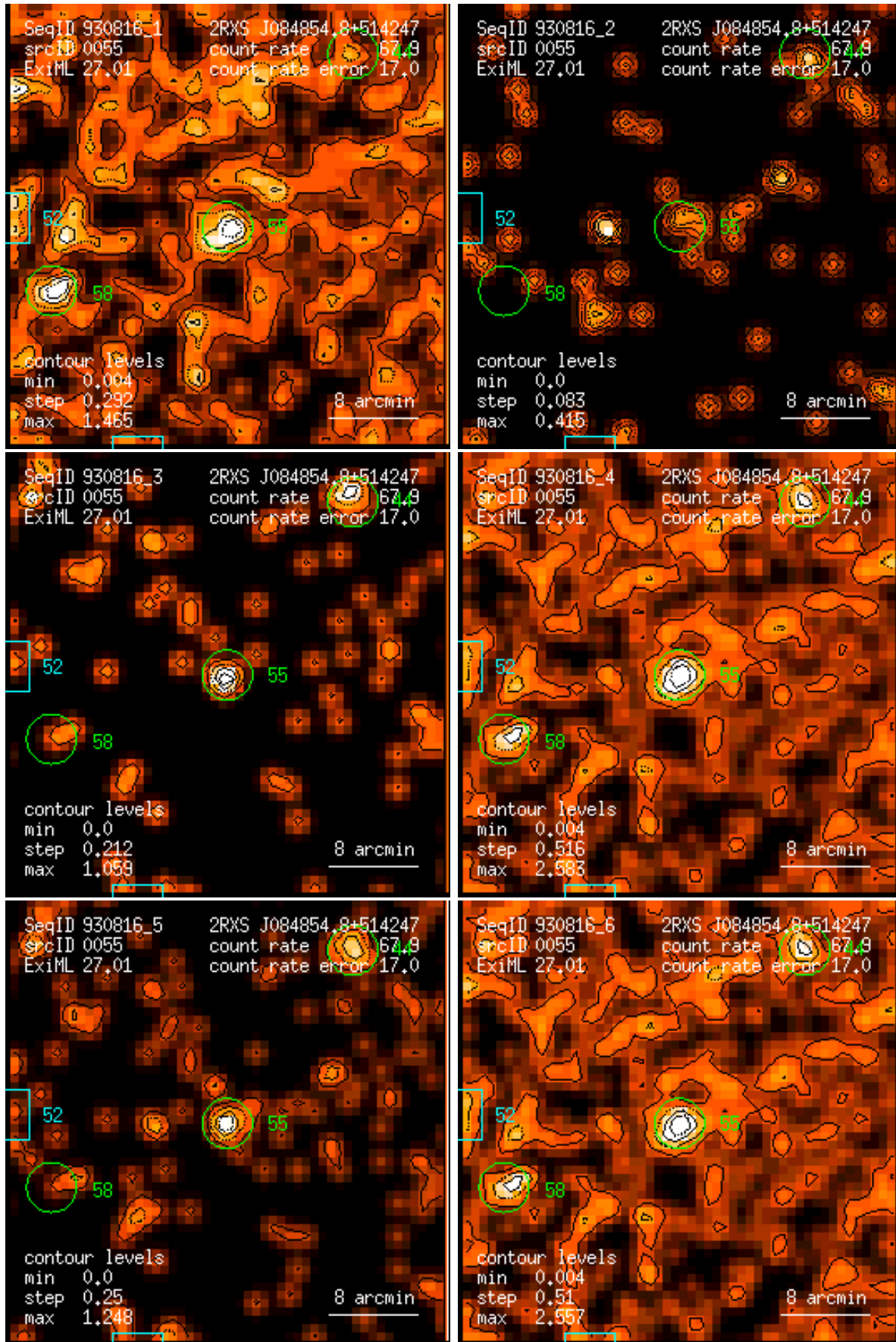
Figure 55: RASS 930816: detection 0055: band rate images, Gaussian filter: (1) PSPC channels 11 – 41, (2) 52 – 90, (3) 91 – 201, (4) 11 – 235, (5) 52 – 201, (6) 11 – 201. Broad band rates in counts/ks. Band rate contour levels in counts/ks/arcmin 2 .
