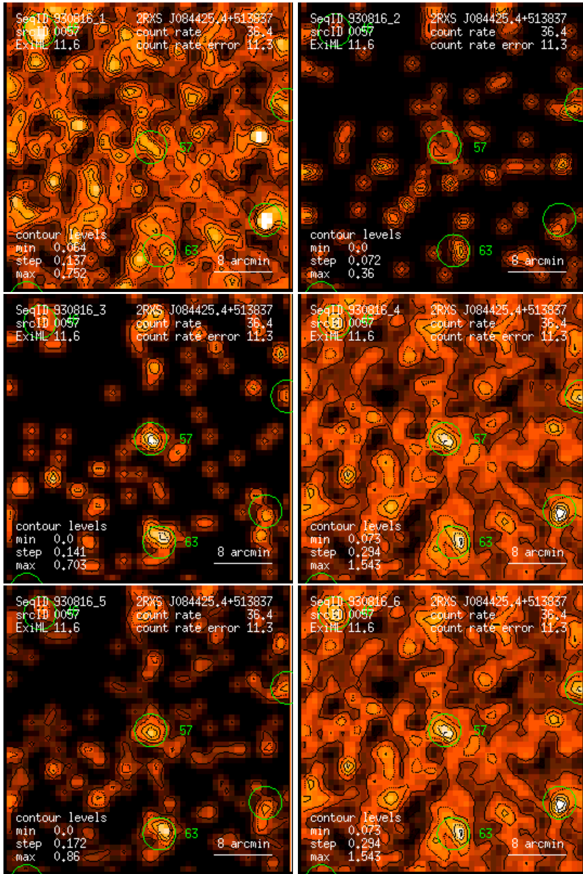
Figure 57: RASS 930816: detection 0057: band rate images, Gaussian filter: (1) PSPC channels 11 – 41, (2) 52 – 90, (3) 91 – 201, (4) 11 – 235, (5) 52 – 201, (6) 11 – 201. Broad band rates in counts/ks. Band rate contour levels in counts/ks/arcmin 2 .
