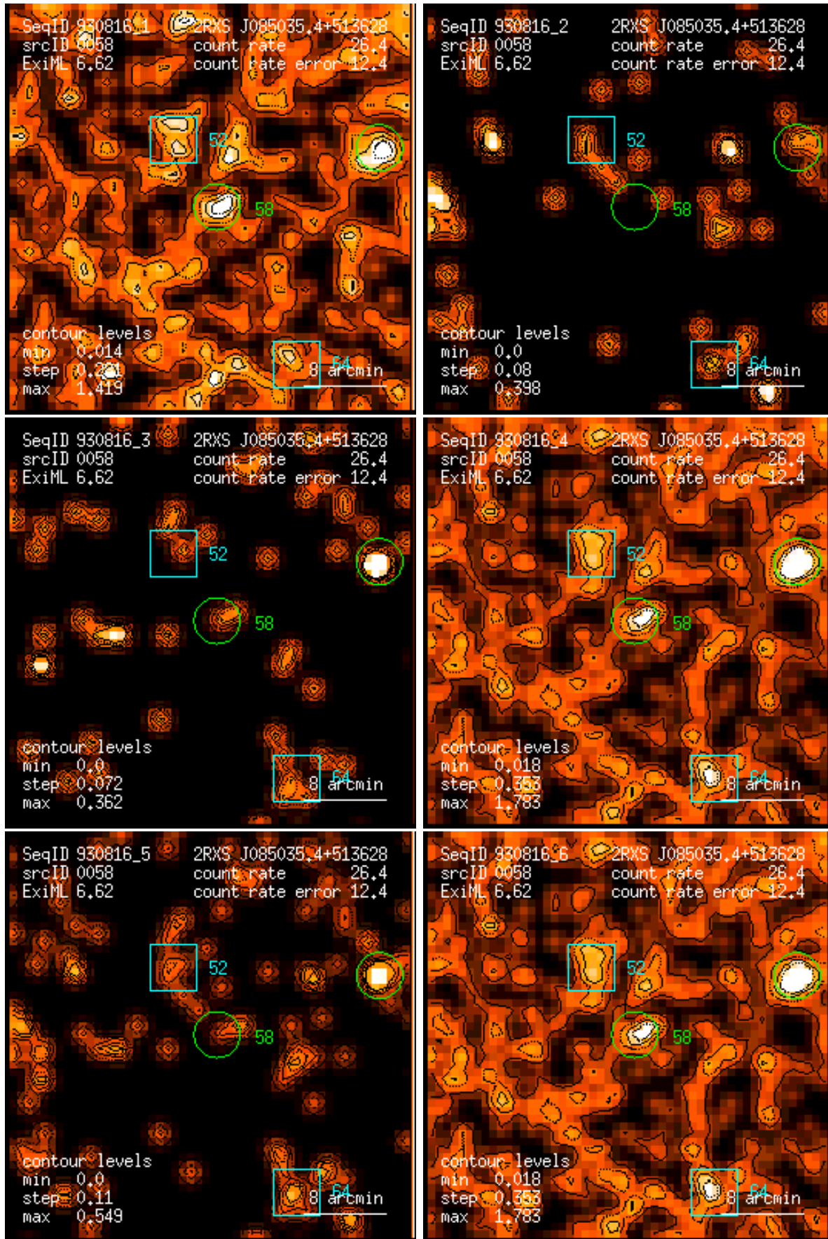
Figure 58: RASS 930816: detection 0058: band rate images, Gaussian filter: (1) PSPC channels 11 – 41, (2) 52 – 90, (3) 91 – 201, (4) 11 – 235, (5) 52 – 201, (6) 11 – 201. Broad band rates in counts/ks. Band rate contour levels in counts/ks/arcmin 2 .
