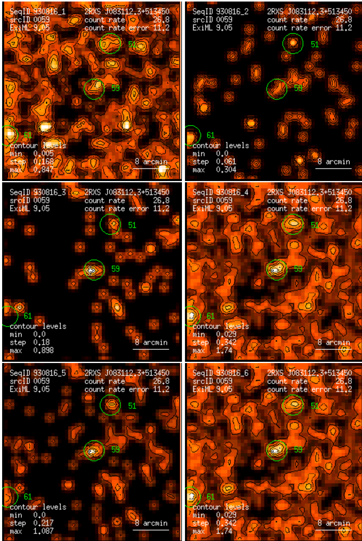
Figure 59: RASS 930816: detection 0059: band rate images, Gaussian filter: (1) PSPC channels 11 – 41, (2) 52 – 90, (3) 91 – 201, (4) 11 – 235, (5) 52 – 201, (6) 11 – 201. Broad band rates in counts/ks. Band rate contour levels in counts/ks/arcmin 2 .
