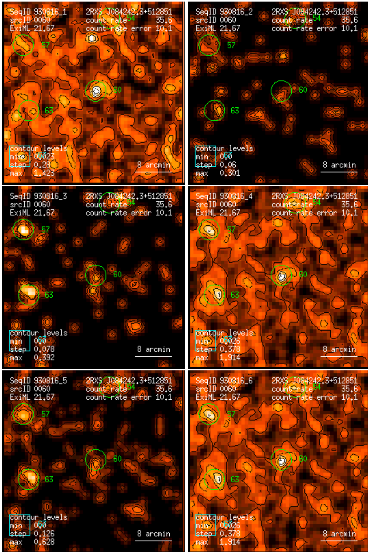
Figure 60: RASS 930816: detection 0060: band rate images, Gaussian filter: (1) PSPC channels 11 – 41, (2) 52 – 90, (3) 91 – 201, (4) 11 – 235, (5) 52 – 201, (6) 11 – 201. Broad band rates in counts/ks. Band rate contour levels in counts/ks/arcmin 2 .
