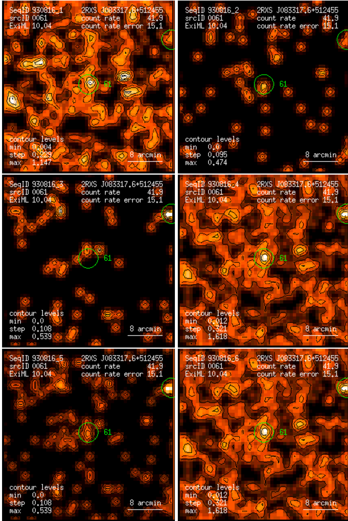
Figure 61: RASS 930816: detection 0061: band rate images, Gaussian filter: (1) PSPC channels 11 – 41, (2) 52 – 90, (3) 91 – 201, (4) 11 – 235, (5) 52 – 201, (6) 11 – 201. Broad band rates in counts/ks. Band rate contour levels in counts/ks/arcmin 2 .
