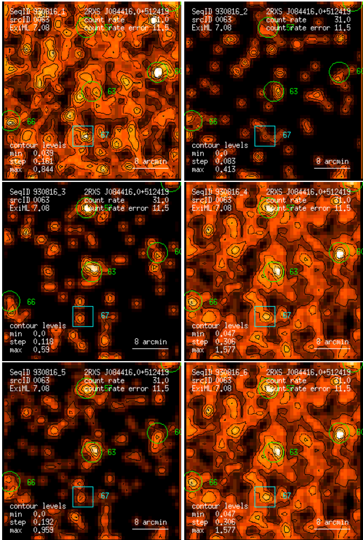
Figure 63: RASS 930816: detection 0063: band rate images, Gaussian filter: (1) PSPC channels 11 – 41, (2) 52 – 90, (3) 91 – 201, (4) 11 – 235, (5) 52 – 201, (6) 11 – 201. Broad band rates in counts/ks. Band rate contour levels in counts/ks/arcmin 2 .
