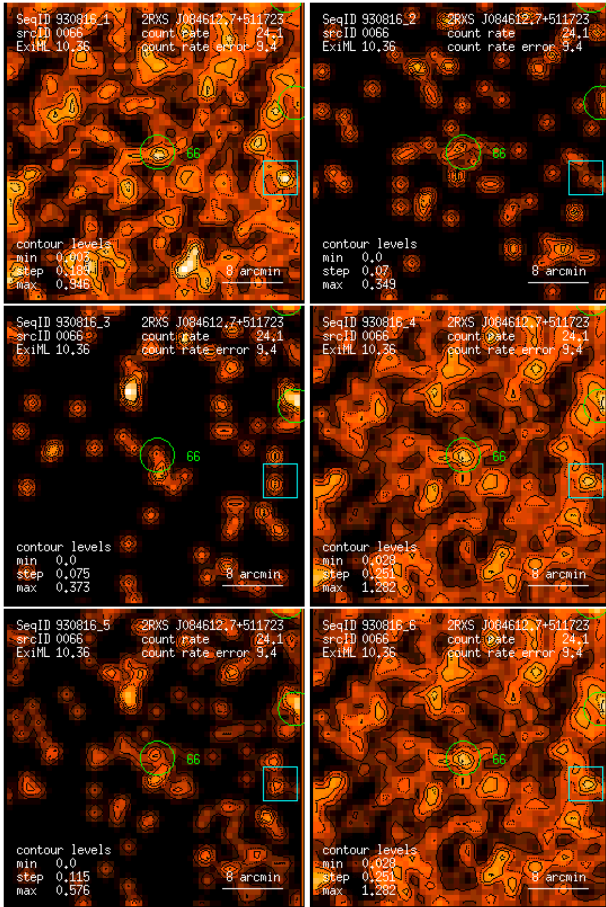
Figure 66: RASS 930816: detection 0066: band rate images, Gaussian filter: (1) PSPC channels 11 – 41, (2) 52 – 90, (3) 91 – 201, (4) 11 – 235, (5) 52 – 201, (6) 11 – 201. Broad band rates in counts/ks. Band rate contour levels in counts/ks/arcmin 2 .
