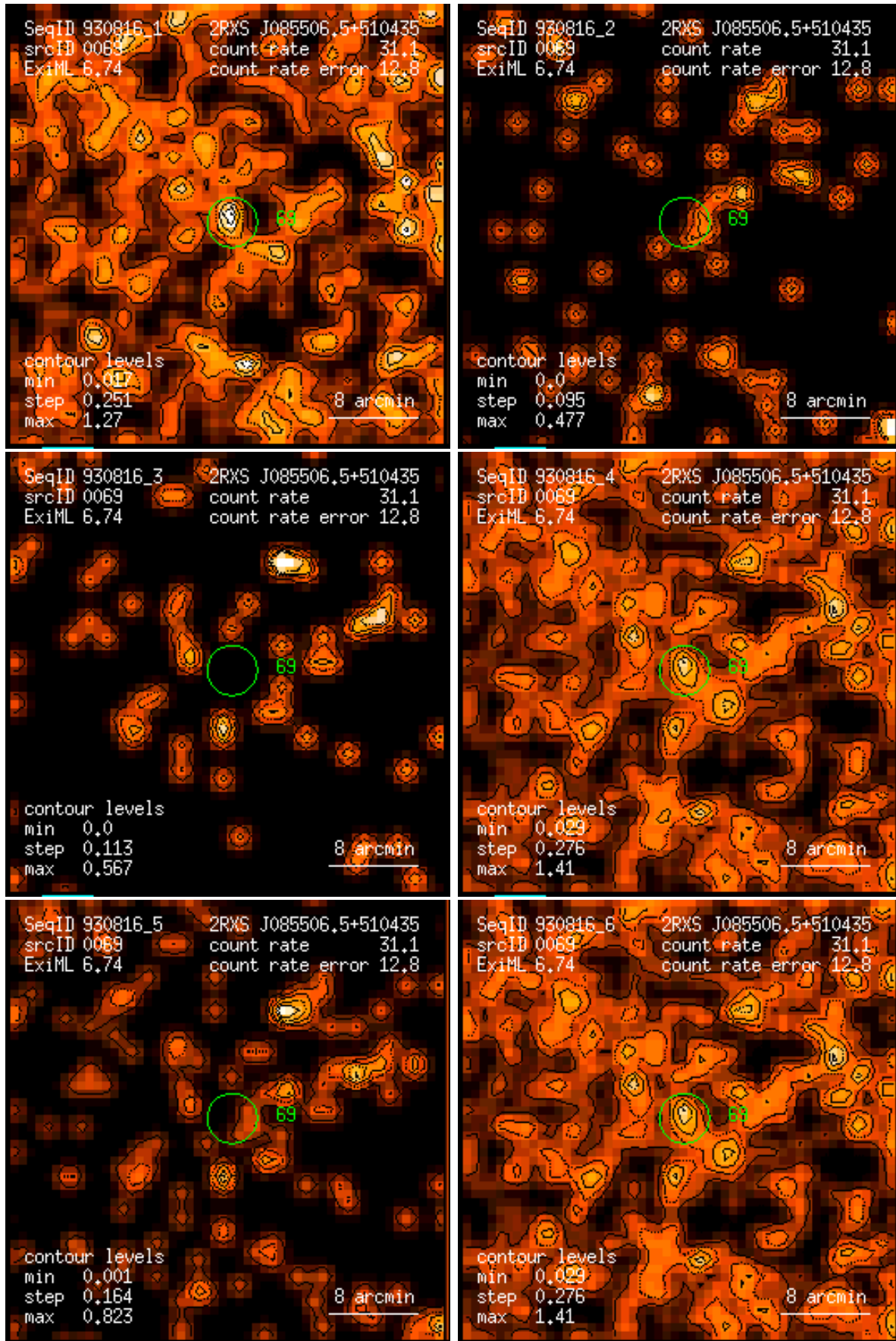
Figure 69: RASS 930816: detection 0069: band rate images, Gaussian filter: (1) PSPC channels 11 – 41, (2) 52 – 90, (3) 91 – 201, (4) 11 – 235, (5) 52 – 201, (6) 11 – 201. Broad band rates in counts/ks. Band rate contour levels in counts/ks/arcmin 2 .
